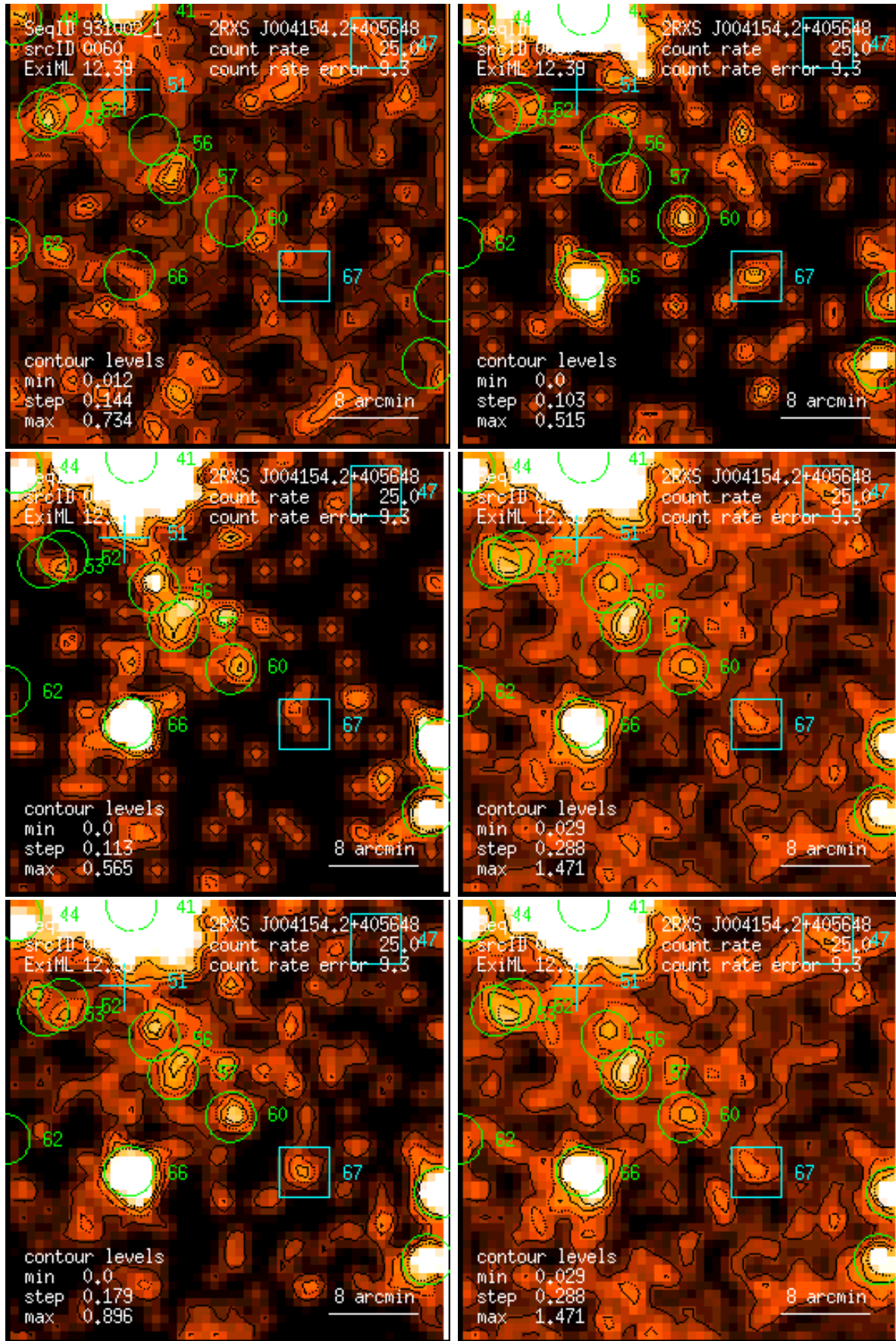
Figure 60: RASS 931002: detection 0060: band rate images, Gaussian filter: (1) PSPC channels 11 – 41, (2) 52 – 90, (3) 91 – 201, (4) 11 – 235, (5) 52 – 201, (6) 11 – 201. Broad band rates in counts/ks. Band rate contour levels in counts/ks/arcmin 2 .
