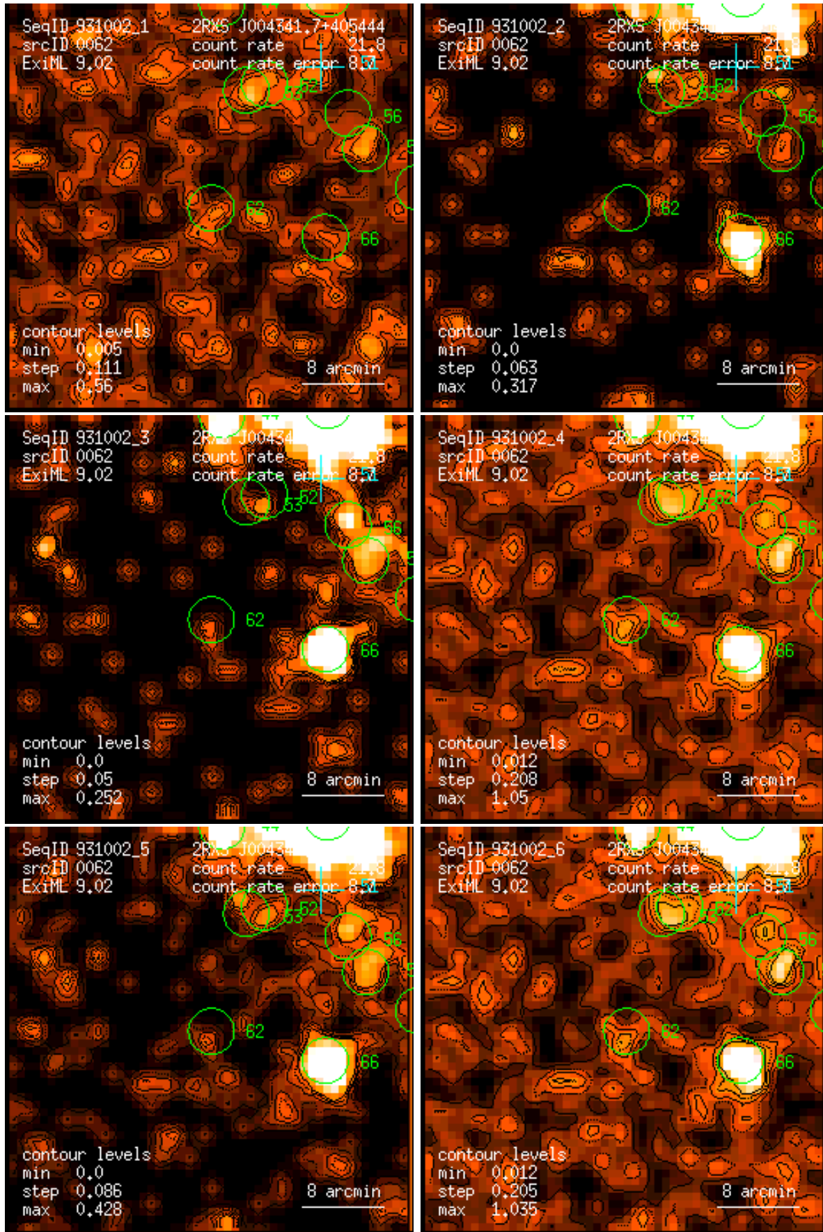
Figure 62: RASS 931002: detection 0062: band rate images, Gaussian filter: (1) PSPC channels 11 – 41, (2) 52 – 90, (3) 91 – 201, (4) 11 – 235, (5) 52 – 201, (6) 11 – 201. Broad band rates in counts/ks. Band rate contour levels in counts/ks/arcmin 2 .
