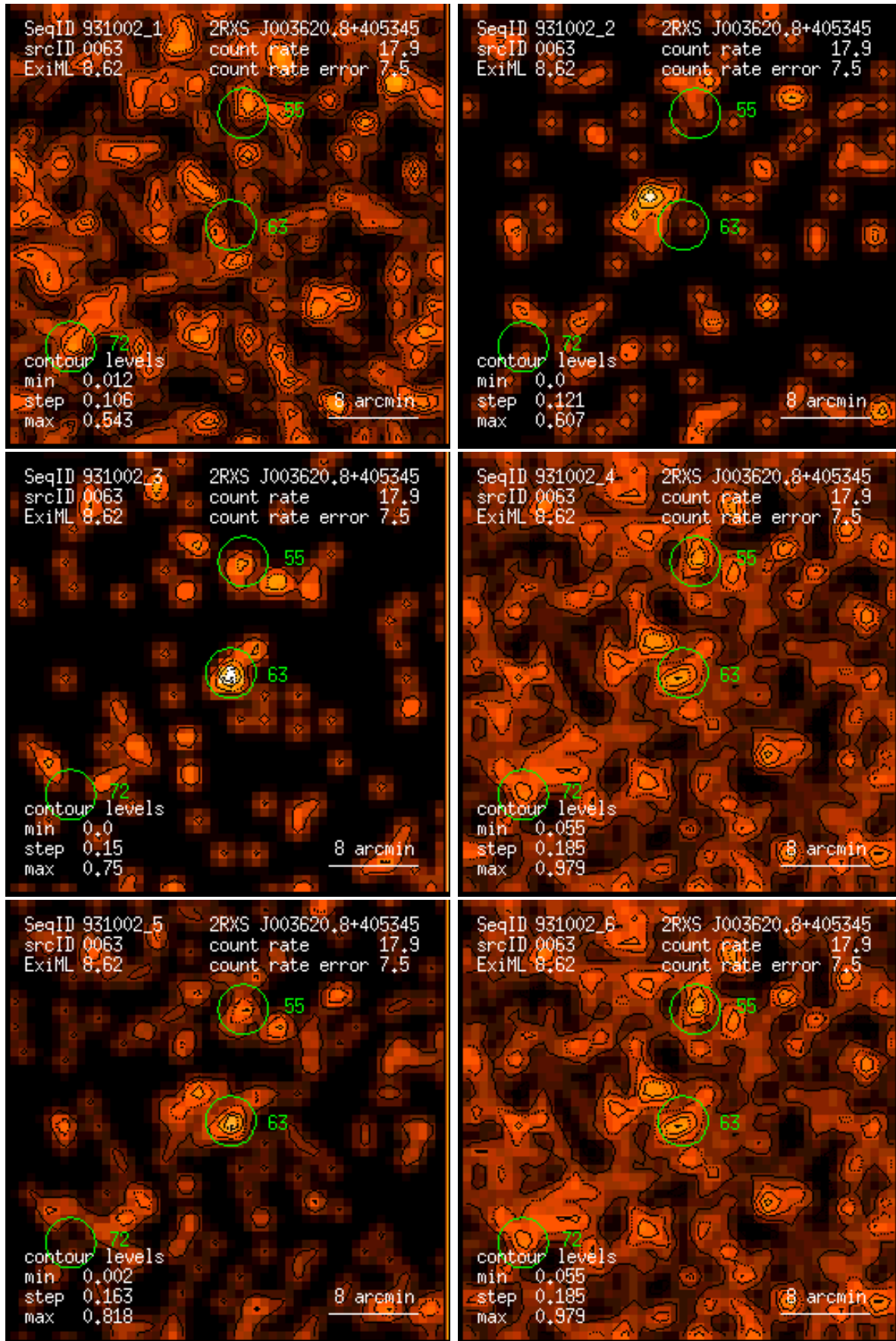
Figure 63: RASS 931002: detection 0063: band rate images, Gaussian filter: (1) PSPC channels 11 – 41, (2) 52 – 90, (3) 91 – 201, (4) 11 – 235, (5) 52 – 201, (6) 11 – 201. Broad band rates in counts/ks. Band rate contour levels in counts/ks/arcmin 2 .
