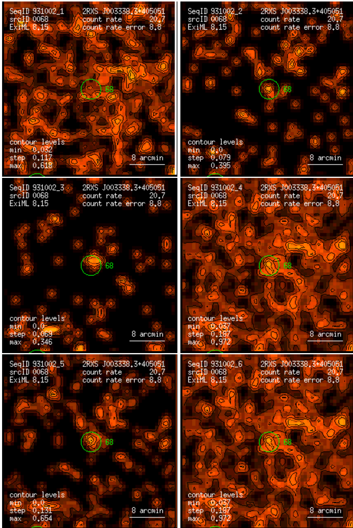
Figure 68: RASS 931002: detection 0068: band rate images, Gaussian filter: (1) PSPC channels 11 – 41, (2) 52 – 90, (3) 91 – 201, (4) 11 – 235, (5) 52 – 201, (6) 11 – 201. Broad band rates in counts/ks. Band rate contour levels in counts/ks/arcmin 2 .
