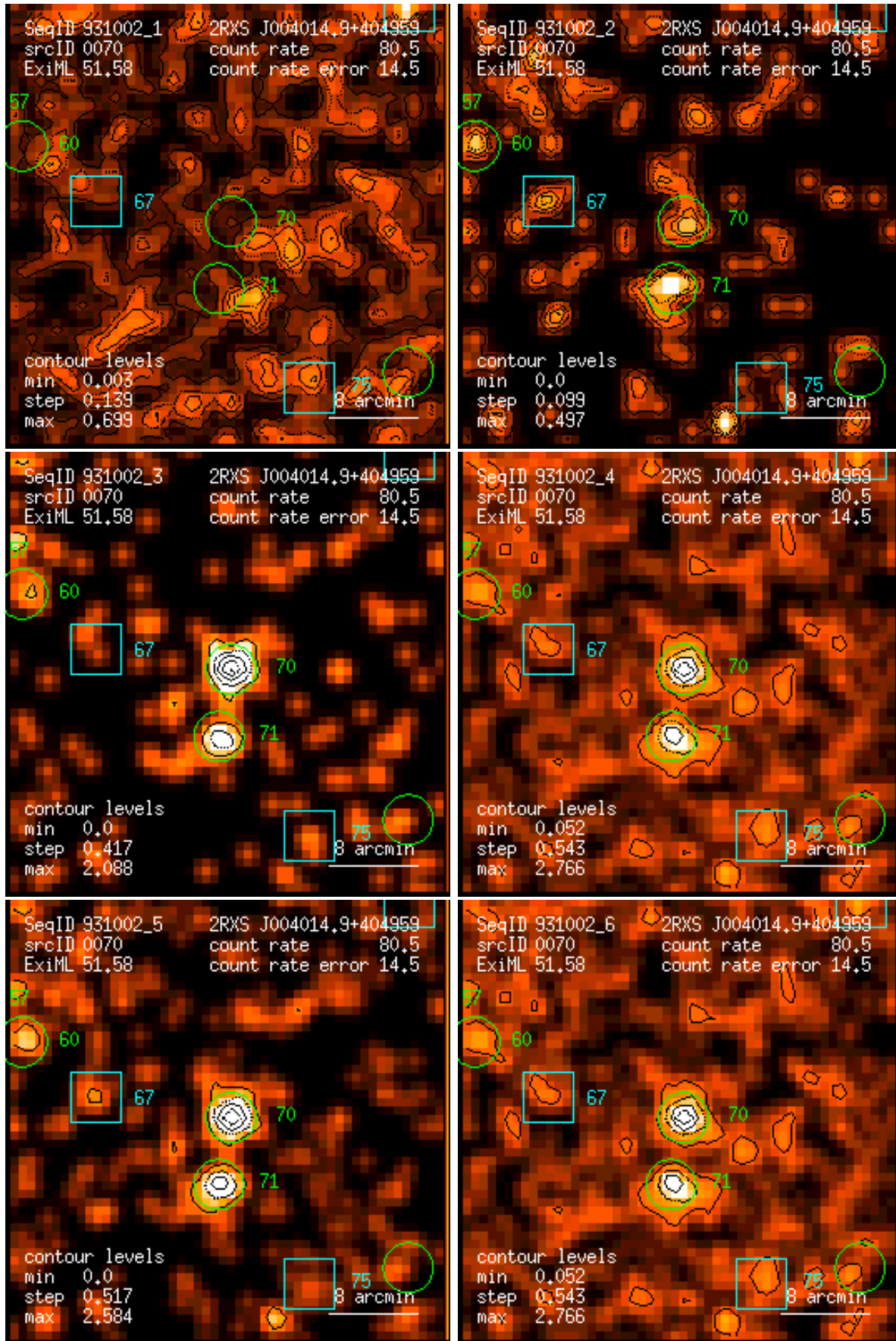
Figure 70: RASS 931002: detection 0070: band rate images, Gaussian filter: (1) PSPC channels 11 – 41, (2) 52 – 90, (3) 91 – 201, (4) 11 – 235, (5) 52 – 201, (6) 11 – 201. Broad band rates in counts/ks. Band rate contour levels in counts/ks/arcmin 2 .
