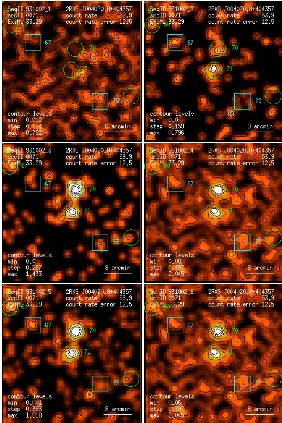
Figure 71: RASS 931002: detection 0071: band rate images, Gaussian filter: (1) PSPC channels 11 – 41, (2) 52 – 90, (3) 91 – 201, (4) 11 – 235, (5) 52 – 201, (6) 11 – 201. Broad band rates in counts/ks. Band rate contour levels in counts/ks/arcmin 2 .
