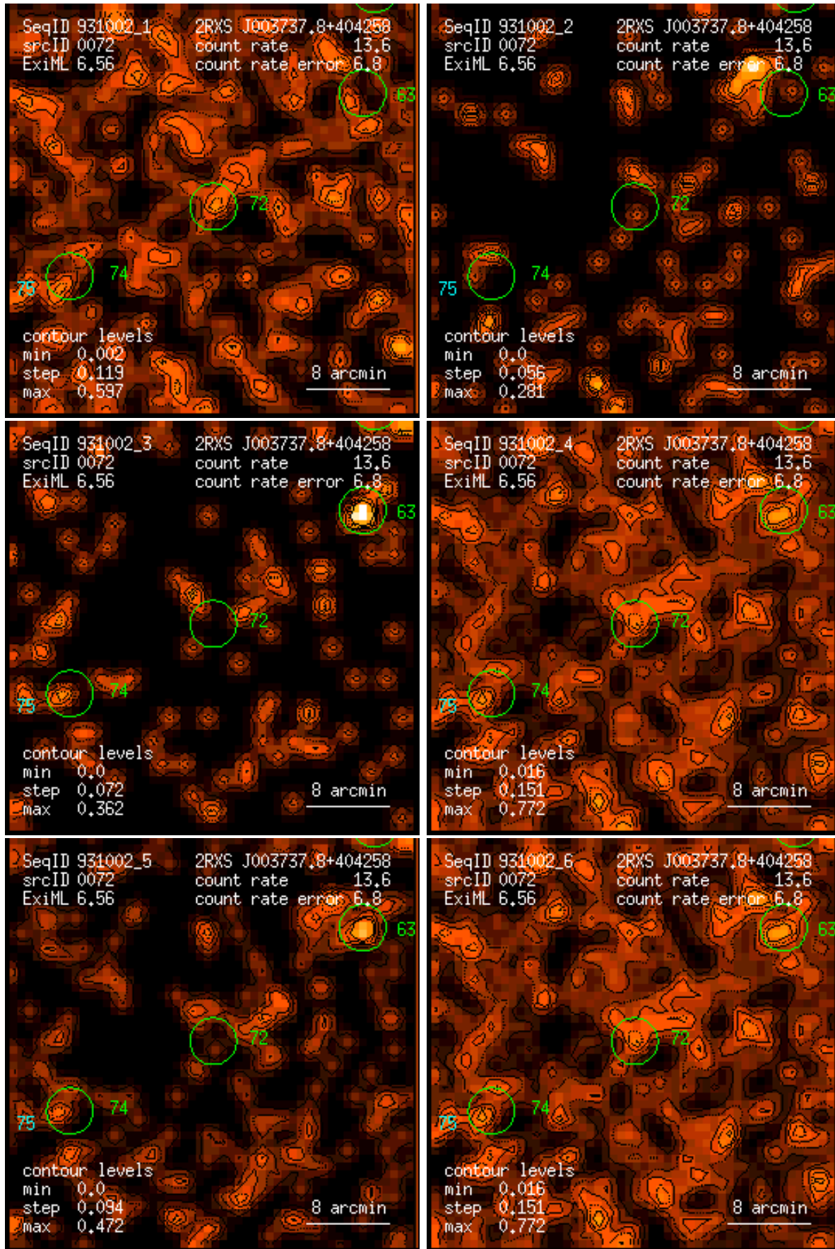
Figure 72: RASS 931002: detection 0072: band rate images, Gaussian filter: (1) PSPC channels 11 – 41, (2) 52 – 90, (3) 91 – 201, (4) 11 – 235, (5) 52 – 201, (6) 11 – 201. Broad band rates in counts/ks. Band rate contour levels in counts/ks/arcmin 2 .
