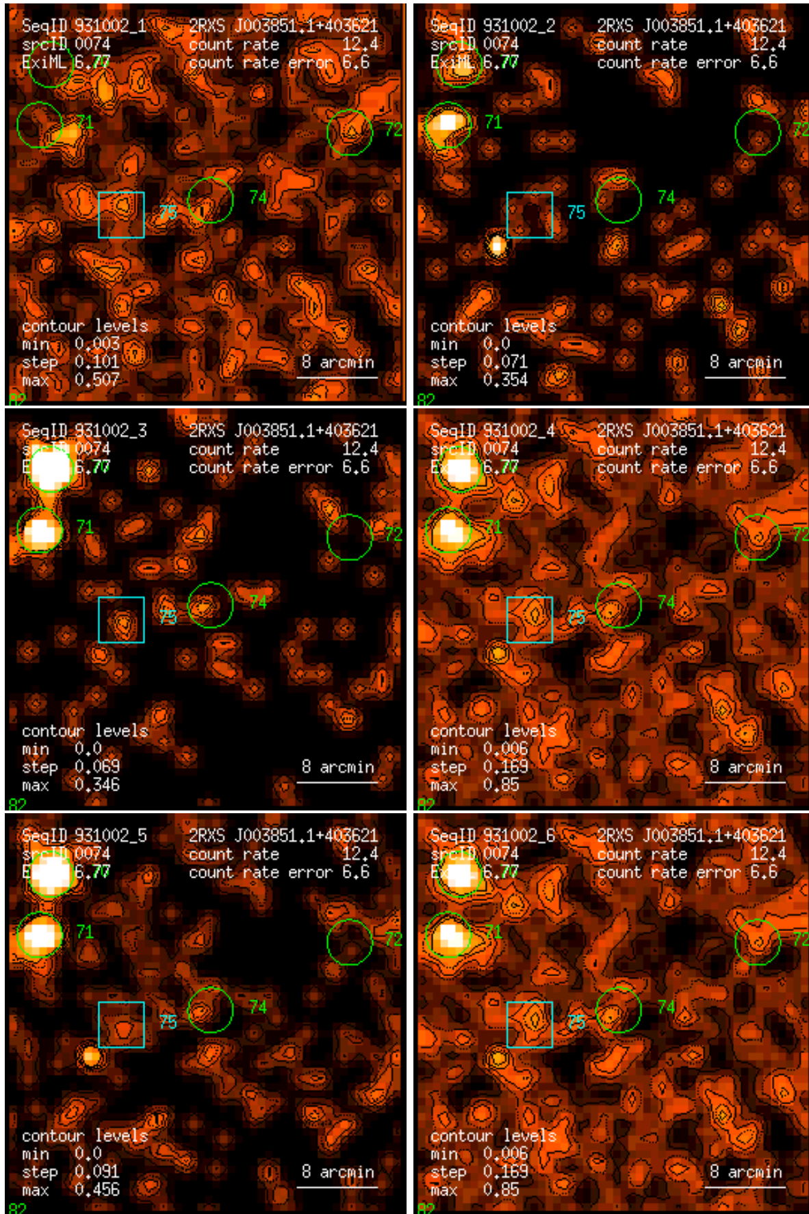
Figure 74: RASS 931002: detection 0074: band rate images, Gaussian filter: (1) PSPC channels 11 – 41, (2) 52 – 90, (3) 91 – 201, (4) 11 – 235, (5) 52 – 201, (6) 11 – 201. Broad band rates in counts/ks. Band rate contour levels in counts/ks/arcmin 2 .
