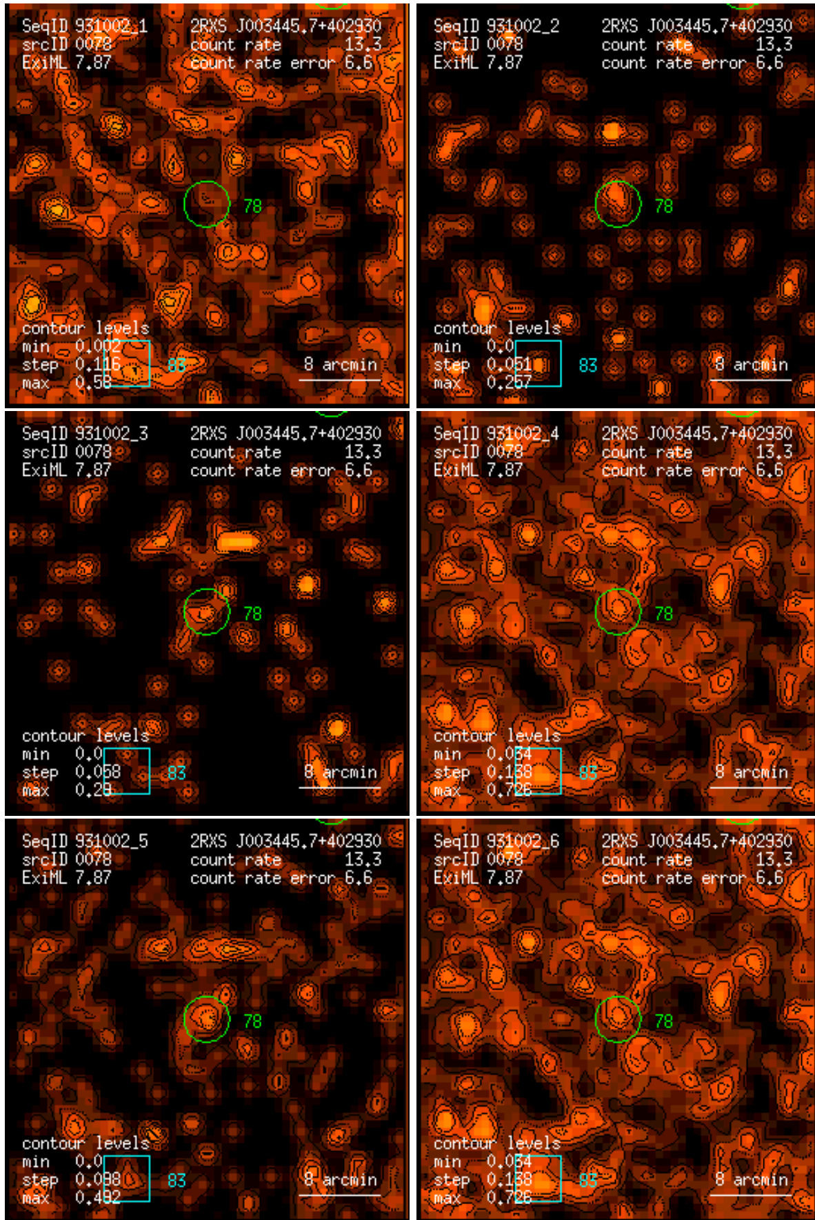
Figure 78: RASS 931002: detection 0078: band rate images, Gaussian filter: (1) PSPC channels 11 – 41, (2) 52 – 90, (3) 91 – 201, (4) 11 – 235, (5) 52 – 201, (6) 11 – 201. Broad band rates in counts/ks. Band rate contour levels in counts/ks/arcmin 2 .
