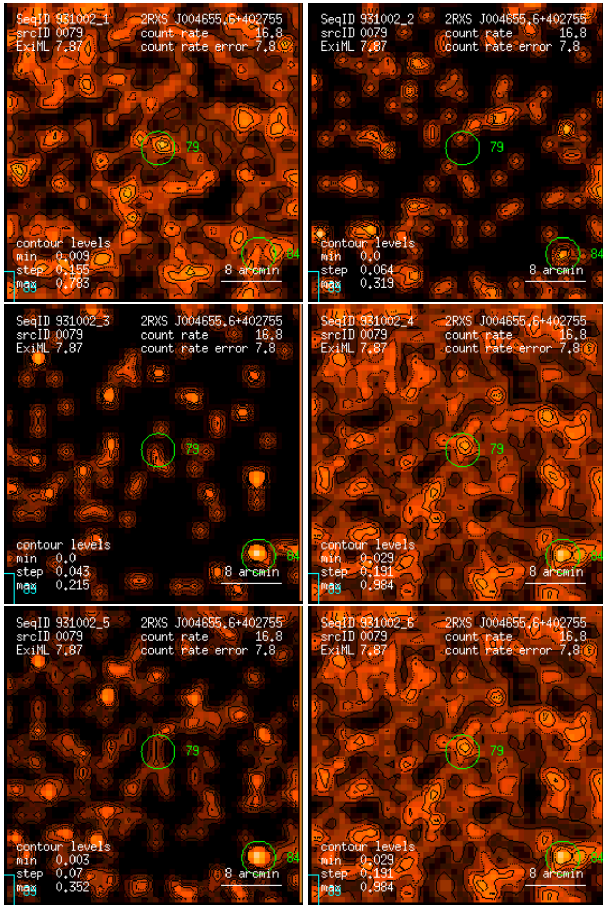
Figure 79: RASS 931002: detection 0079: band rate images, Gaussian filter: (1) PSPC channels 11 – 41, (2) 52 – 90, (3) 91 – 201, (4) 11 – 235, (5) 52 – 201, (6) 11 – 201. Broad band rates in counts/ks. Band rate contour levels in counts/ks/arcmin 2 .
