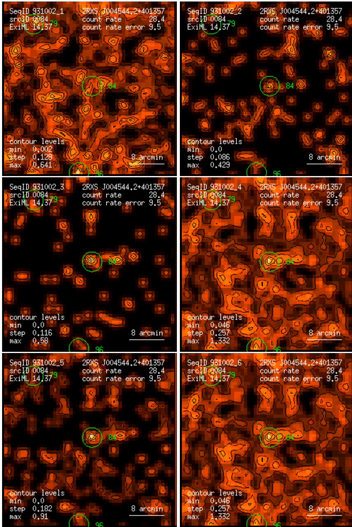
Figure 84: RASS 931002: detection 0084: band rate images, Gaussian filter: (1) PSPC channels 11 – 41, (2) 52 – 90, (3) 91 – 201, (4) 11 – 235, (5) 52 – 201, (6) 11 – 201. Broad band rates in counts/ks. Band rate contour levels in counts/ks/arcmin 2 .
