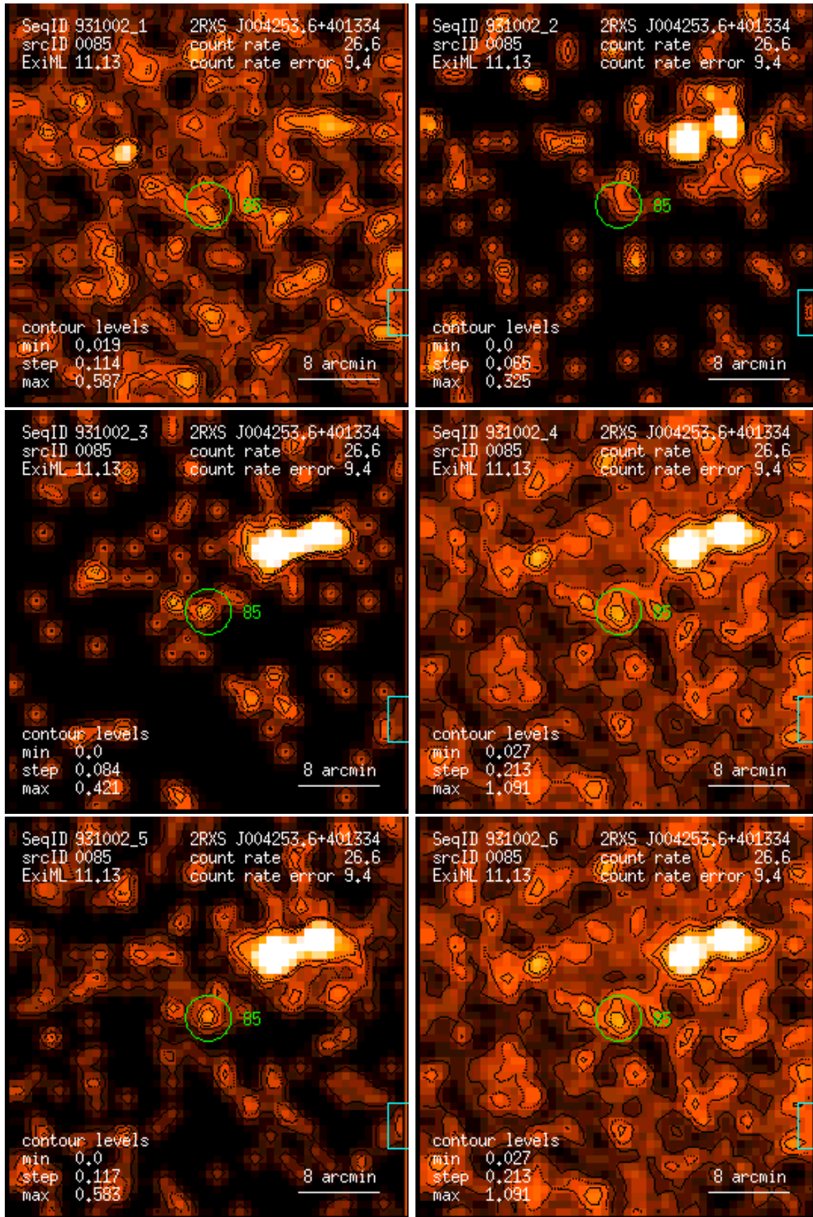
Figure 85: RASS 931002: detection 0085: band rate images, Gaussian filter: (1) PSPC channels 11 – 41, (2) 52 – 90, (3) 91 – 201, (4) 11 – 235, (5) 52 – 201, (6) 11 – 201. Broad band rates in counts/ks. Band rate contour levels in counts/ks/arcmin 2 .
