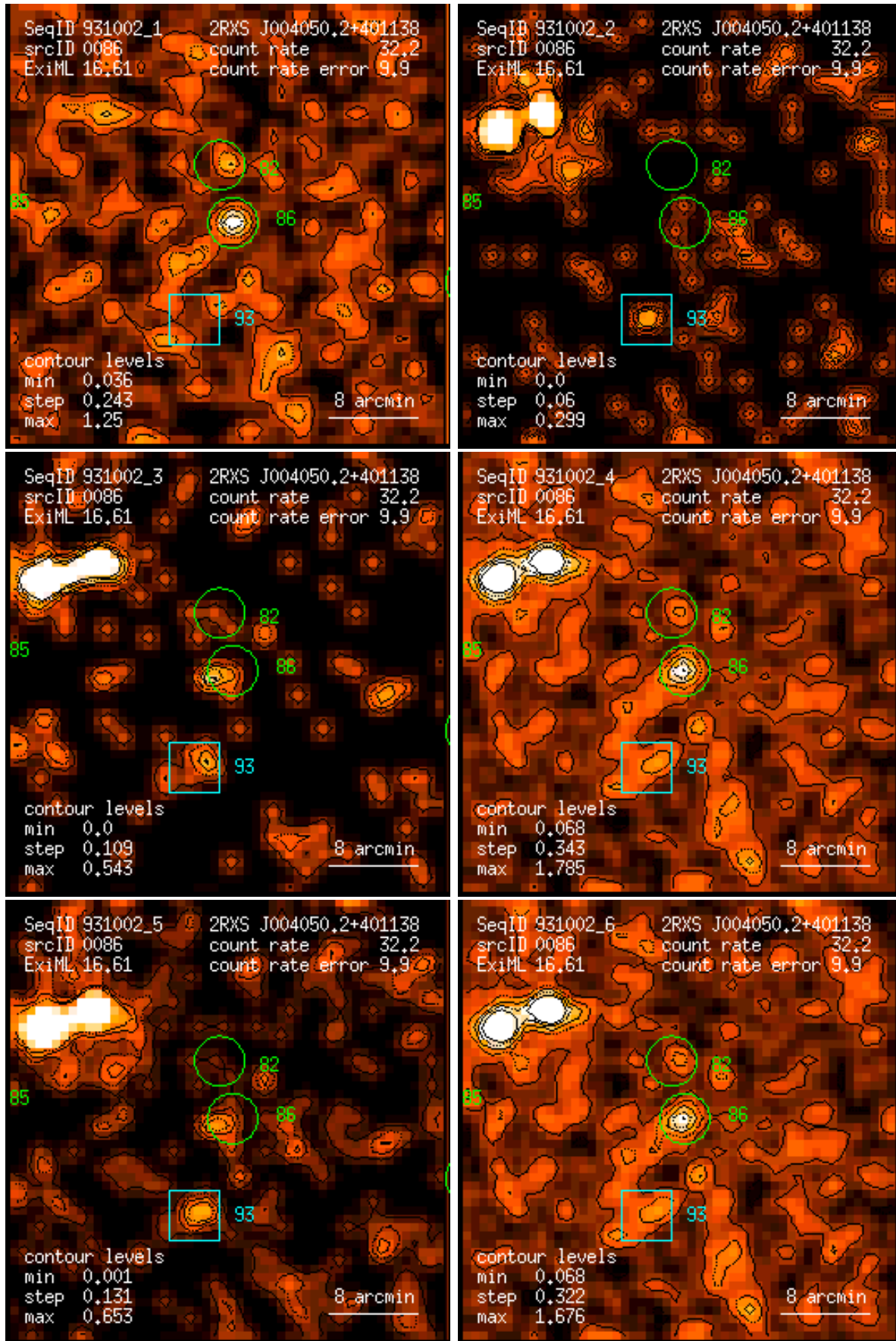
Figure 86: RASS 931002: detection 0086: band rate images, Gaussian filter: (1) PSPC channels 11 – 41, (2) 52 – 90, (3) 91 – 201, (4) 11 – 235, (5) 52 – 201, (6) 11 – 201. Broad band rates in counts/ks. Band rate contour levels in counts/ks/arcmin 2 .
