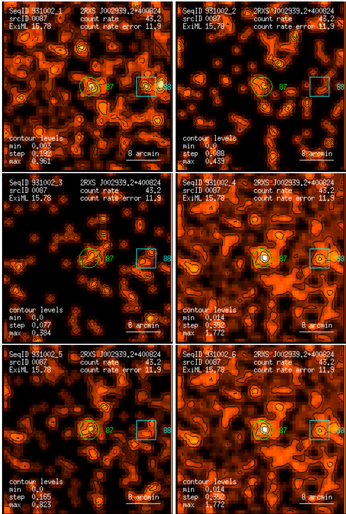
Figure 87: RASS 931002: detection 0087: band rate images, Gaussian filter: (1) PSPC channels 11 – 41, (2) 52 – 90, (3) 91 – 201, (4) 11 – 235, (5) 52 – 201, (6) 11 – 201. Broad band rates in counts/ks. Band rate contour levels in counts/ks/arcmin 2 .
