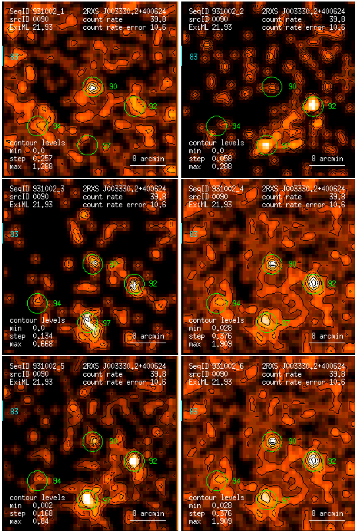
Figure 90: RASS 931002: detection 0090: band rate images, Gaussian filter: (1) PSPC channels 11 – 41, (2) 52 – 90, (3) 91 – 201, (4) 11 – 235, (5) 52 – 201, (6) 11 – 201. Broad band rates in counts/ks. Band rate contour levels in counts/ks/arcmin 2 .
