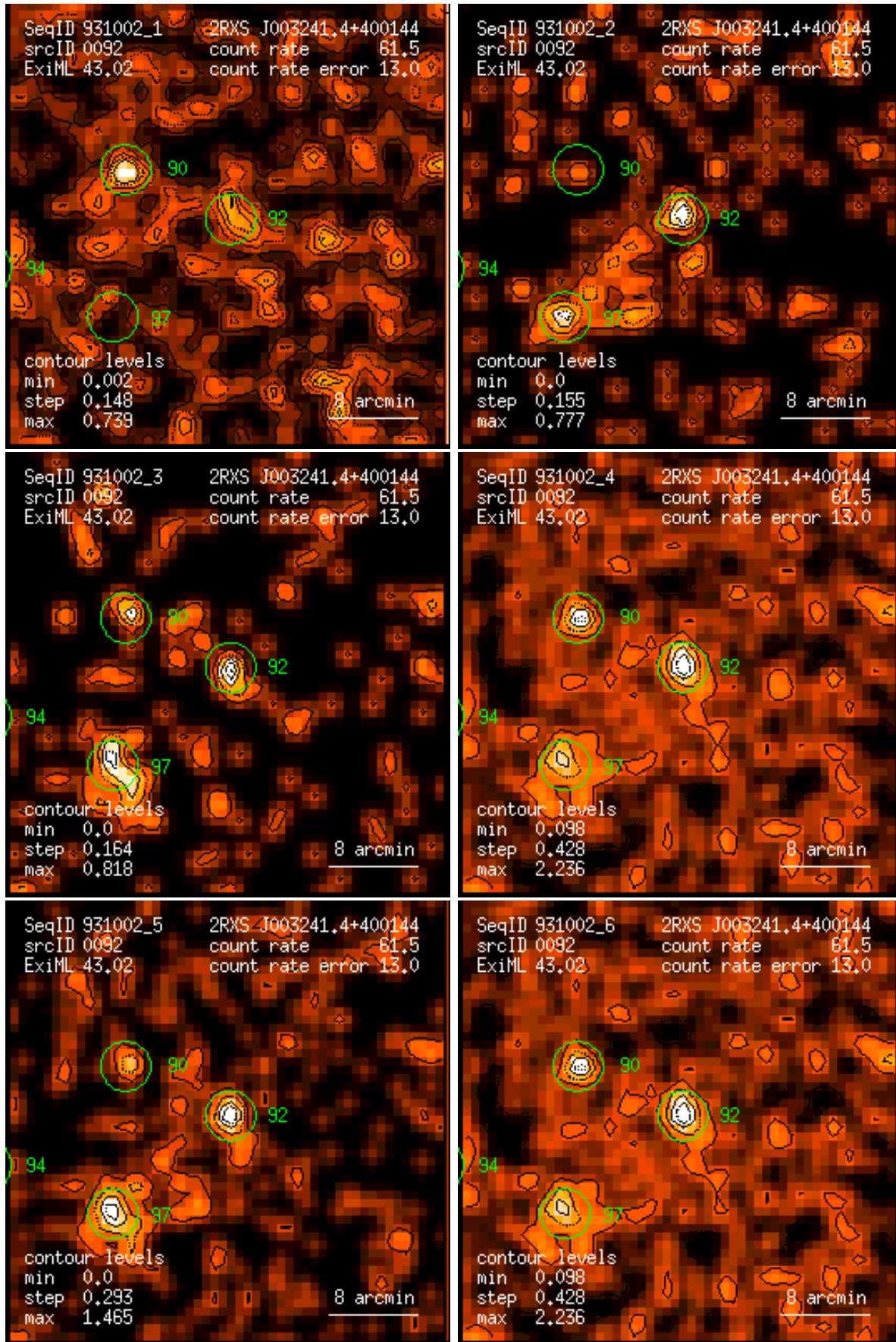
Figure 92: RASS 931002: detection 0092: band rate images, Gaussian filter: (1) PSPC channels 11 – 41, (2) 52 – 90, (3) 91 – 201, (4) 11 – 235, (5) 52 – 201, (6) 11 – 201. Broad band rates in counts/ks. Band rate contour levels in counts/ks/arcmin 2 .
