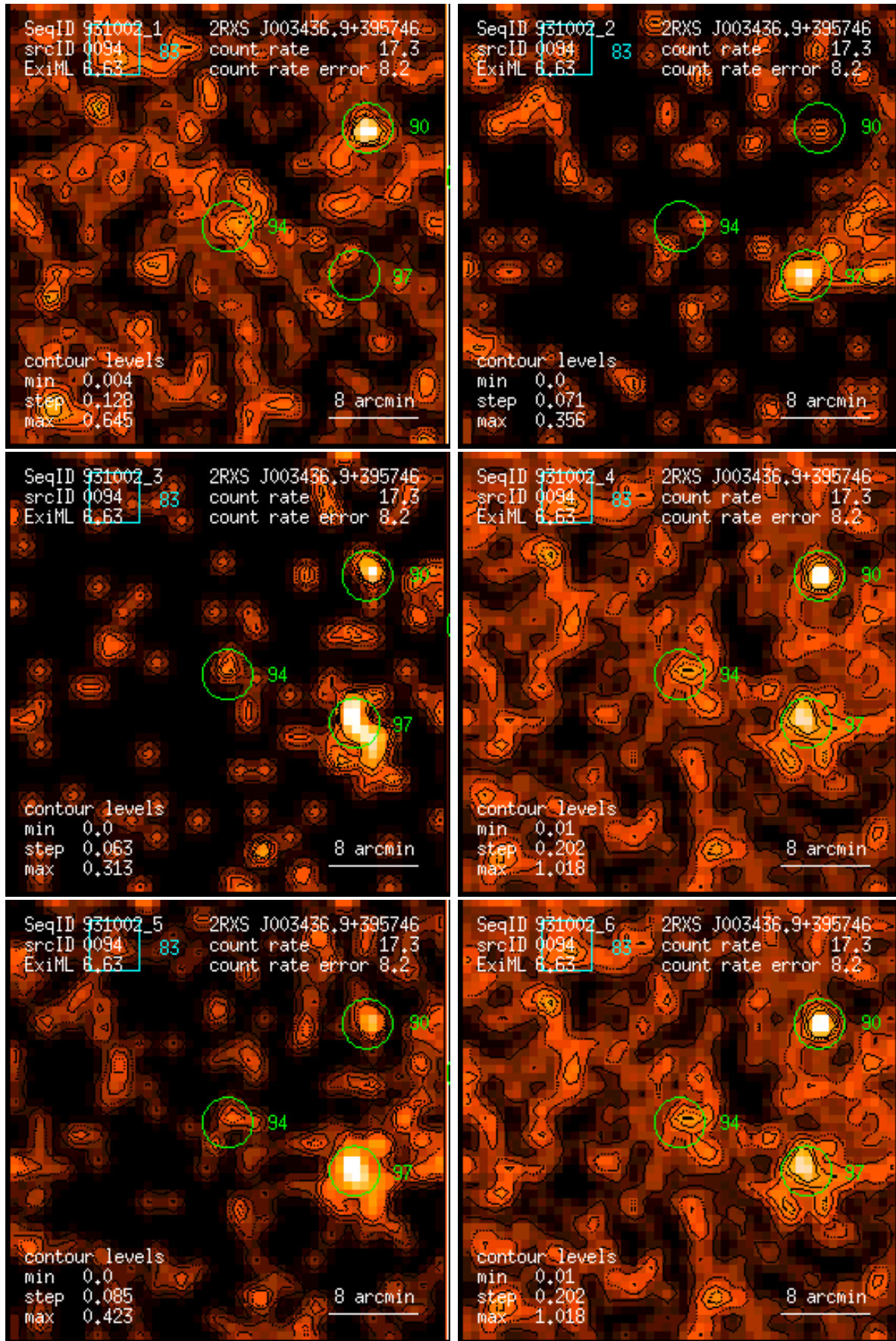
Figure 94: RASS 931002: detection 0094: band rate images, Gaussian filter: (1) PSPC channels 11 – 41, (2) 52 – 90, (3) 91 – 201, (4) 11 – 235, (5) 52 – 201, (6) 11 – 201. Broad band rates in counts/ks. Band rate contour levels in counts/ks/arcmin 2 .
