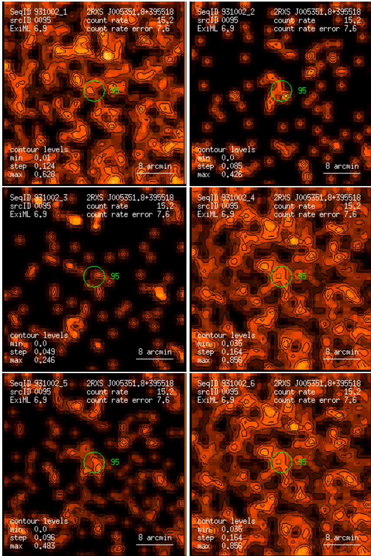
Figure 95: RASS 931002: detection 0095: band rate images, Gaussian filter: (1) PSPC channels 11 – 41, (2) 52 – 90, (3) 91 – 201, (4) 11 – 235, (5) 52 – 201, (6) 11 – 201. Broad band rates in counts/ks. Band rate contour levels in counts/ks/arcmin 2 .
