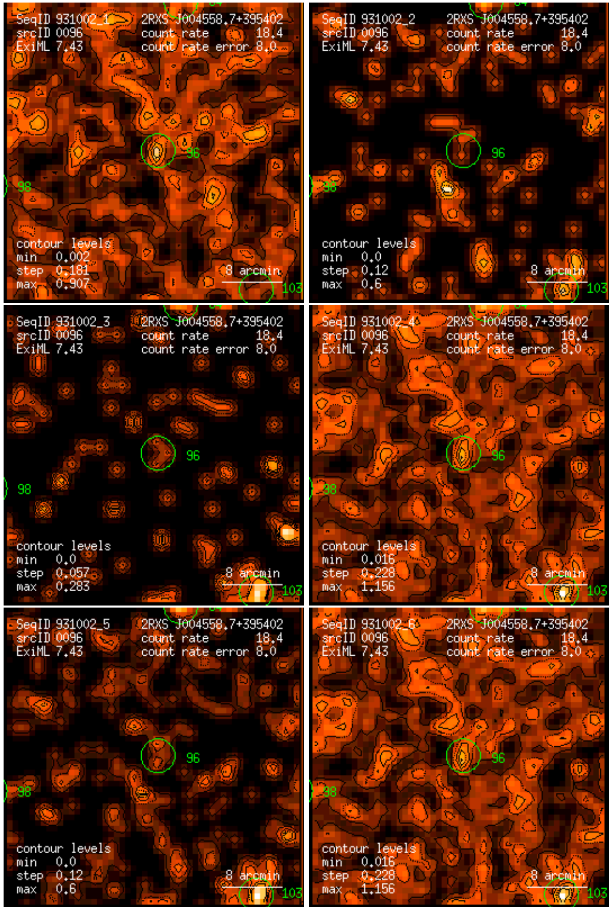
Figure 96: RASS 931002: detection 0096: band rate images, Gaussian filter: (1) PSPC channels 11 – 41, (2) 52 – 90, (3) 91 – 201, (4) 11 – 235, (5) 52 – 201, (6) 11 – 201. Broad band rates in counts/ks. Band rate contour levels in counts/ks/arcmin 2 .
