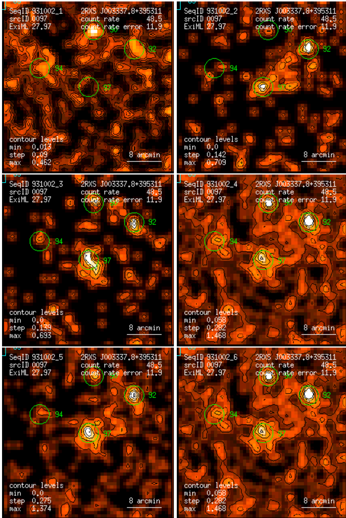
Figure 97: RASS 931002: detection 0097: band rate images, Gaussian filter: (1) PSPC channels 11 – 41, (2) 52 – 90, (3) 91 – 201, (4) 11 – 235, (5) 52 – 201, (6) 11 – 201. Broad band rates in counts/ks. Band rate contour levels in counts/ks/arcmin 2 .
