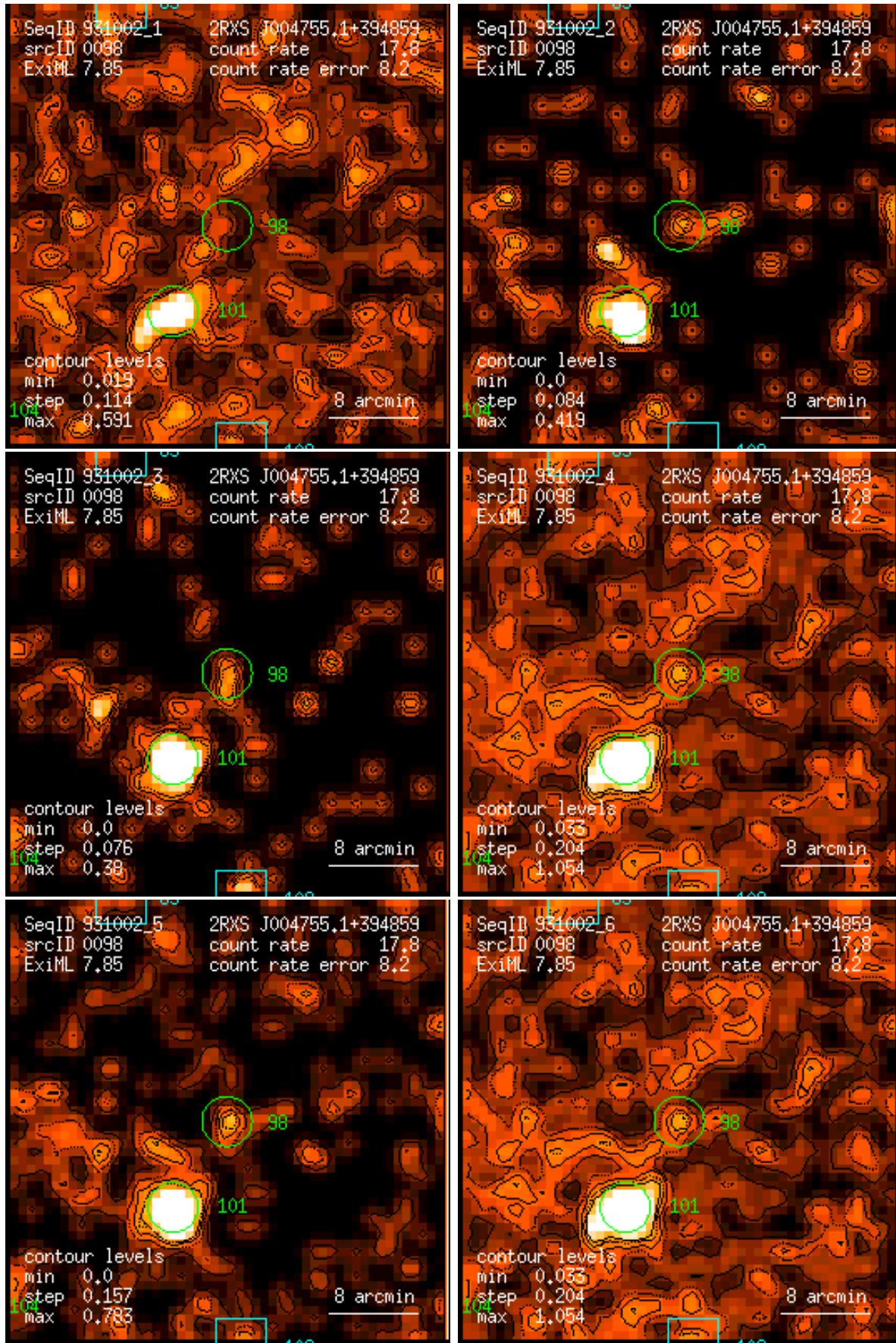
Figure 98: RASS 931002: detection 0098: band rate images, Gaussian filter: (1) PSPC channels 11 – 41, (2) 52 – 90, (3) 91 – 201, (4) 11 – 235, (5) 52 – 201, (6) 11 – 201. Broad band rates in counts/ks. Band rate contour levels in counts/ks/arcmin 2 .
