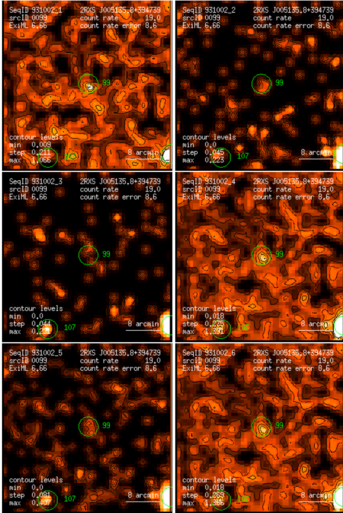
Figure 99: RASS 931002: detection 0099: band rate images, Gaussian filter: (1) PSPC channels 11 – 41, (2) 52 – 90, (3) 91 – 201, (4) 11 – 235, (5) 52 – 201, (6) 11 – 201. Broad band rates in counts/ks. Band rate contour levels in counts/ks/arcmin 2 .
