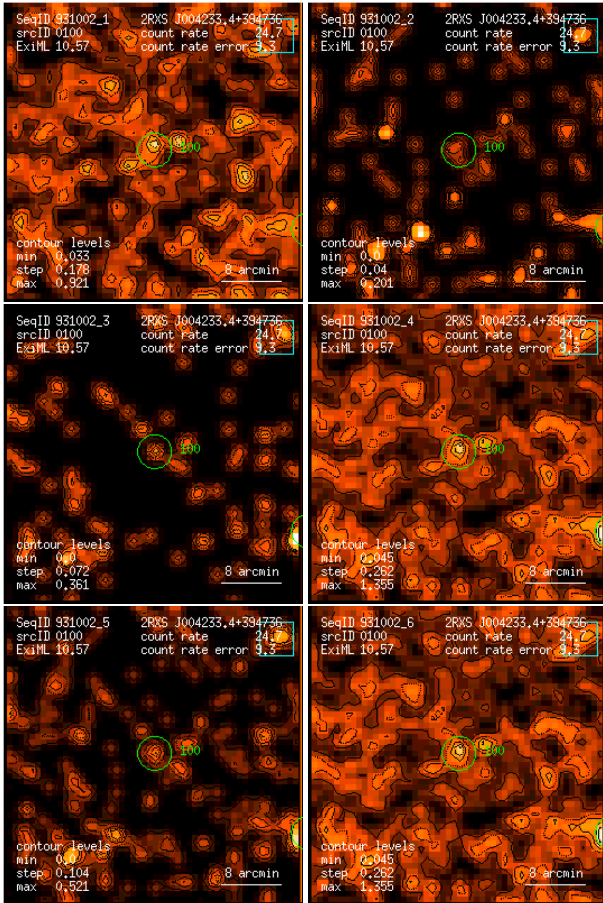
Figure 100: RASS 931002: detection 0100: band rate images, Gaussian filter: (1) PSPC channels 11 – 41, (2) 52 – 90, (3) 91 – 201, (4) 11 – 235, (5) 52 – 201, (6) 11 – 201. Broad band rates in counts/ks. Band rate contour levels in counts/ks/arcmin 2 .
