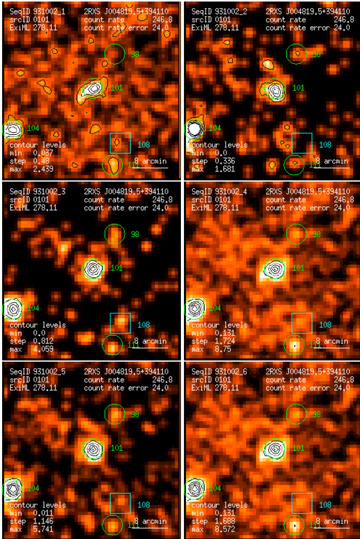
Figure 101: RASS 931002: detection 0101: band rate images, Gaussian filter: (1) PSPC channels 11 – 41, (2) 52 – 90, (3) 91 – 201, (4) 11 – 235, (5) 52 – 201, (6) 11 – 201. Broad band rates in counts/ks. Band rate contour levels in counts/ks/arcmin 2 .
