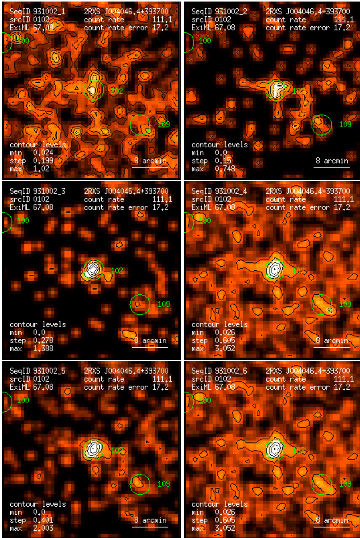
Figure 102: RASS 931002: detection 0102: band rate images, Gaussian filter: (1) PSPC channels 11 – 41, (2) 52 – 90, (3) 91 – 201, (4) 11 – 235, (5) 52 – 201, (6) 11 – 201. Broad band rates in counts/ks. Band rate contour levels in counts/ks/arcmin 2 .
