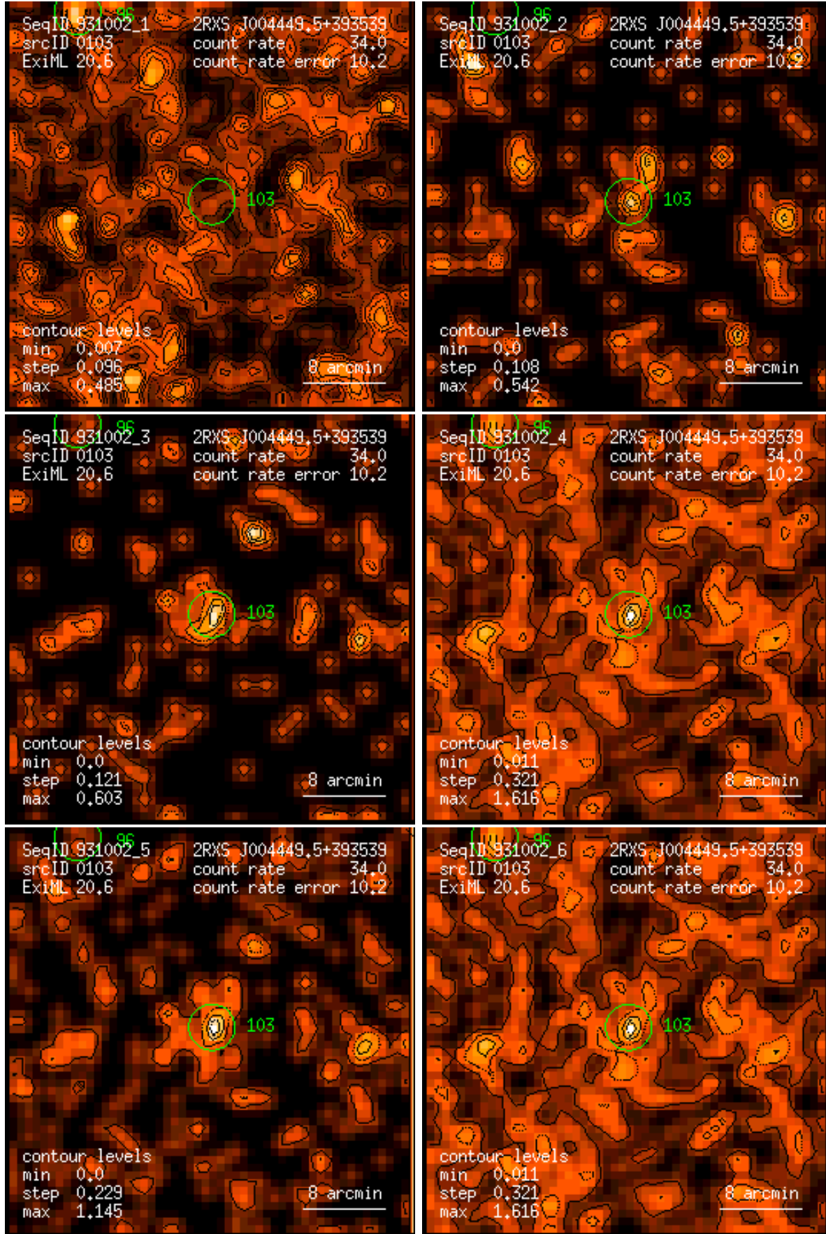
Figure 103: RASS 931002: detection 0103: band rate images, Gaussian filter: (1) PSPC channels 11 – 41, (2) 52 – 90, (3) 91 – 201, (4) 11 – 235, (5) 52 – 201, (6) 11 – 201. Broad band rates in counts/ks. Band rate contour levels in counts/ks/arcmin 2 .
