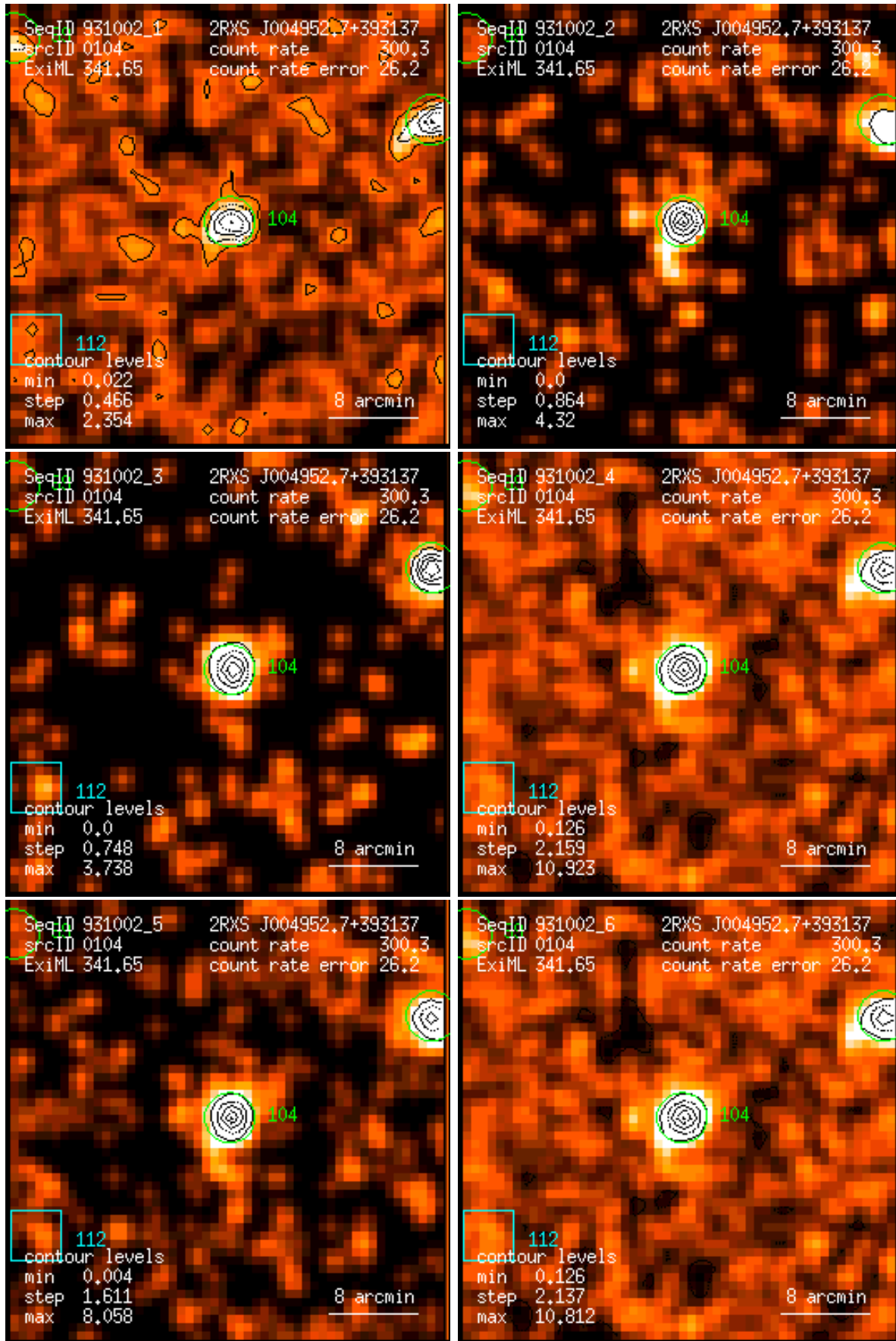
Figure 104: RASS 931002: detection 0104: band rate images, Gaussian filter: (1) PSPC channels 11 – 41, (2) 52 – 90, (3) 91 – 201, (4) 11 – 235, (5) 52 – 201, (6) 11 – 201. Broad band rates in counts/ks. Band rate contour levels in counts/ks/arcmin 2 .
