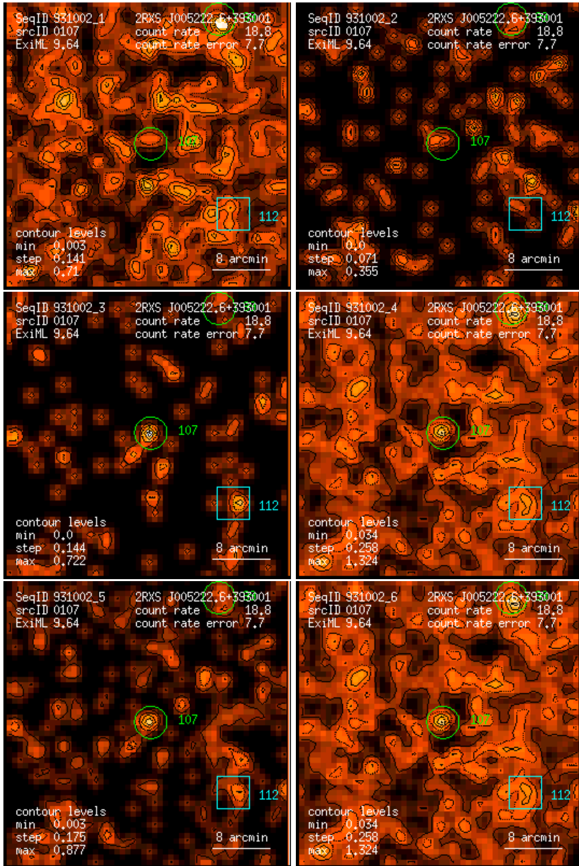
Figure 107: RASS 931002: detection 0107: band rate images, Gaussian filter: (1) PSPC channels 11 – 41, (2) 52 – 90, (3) 91 – 201, (4) 11 – 235, (5) 52 – 201, (6) 11 – 201. Broad band rates in counts/ks. Band rate contour levels in counts/ks/arcmin 2 .
