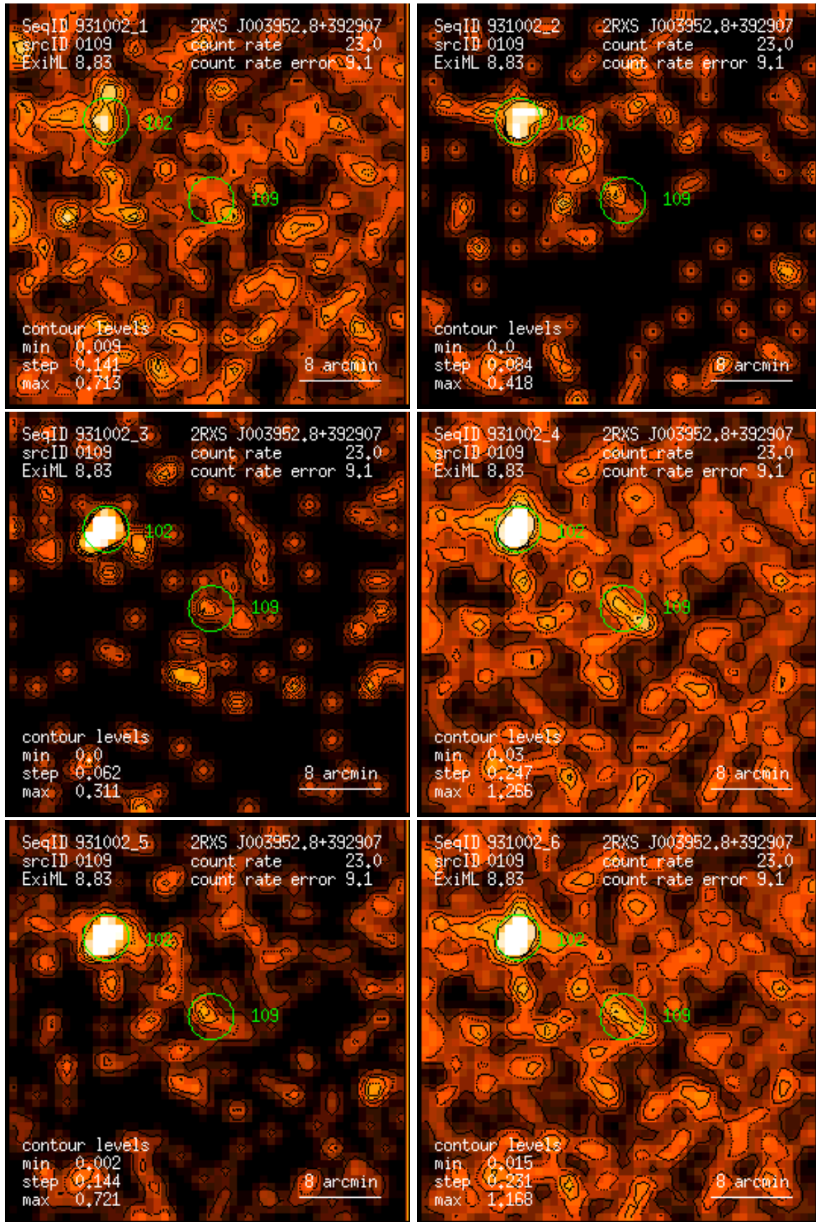
Figure 109: RASS 931002: detection 0109: band rate images, Gaussian filter: (1) PSPC channels 11 – 41, (2) 52 – 90, (3) 91 – 201, (4) 11 – 235, (5) 52 – 201, (6) 11 – 201. Broad band rates in counts/ks. Band rate contour levels in counts/ks/arcmin 2 .
