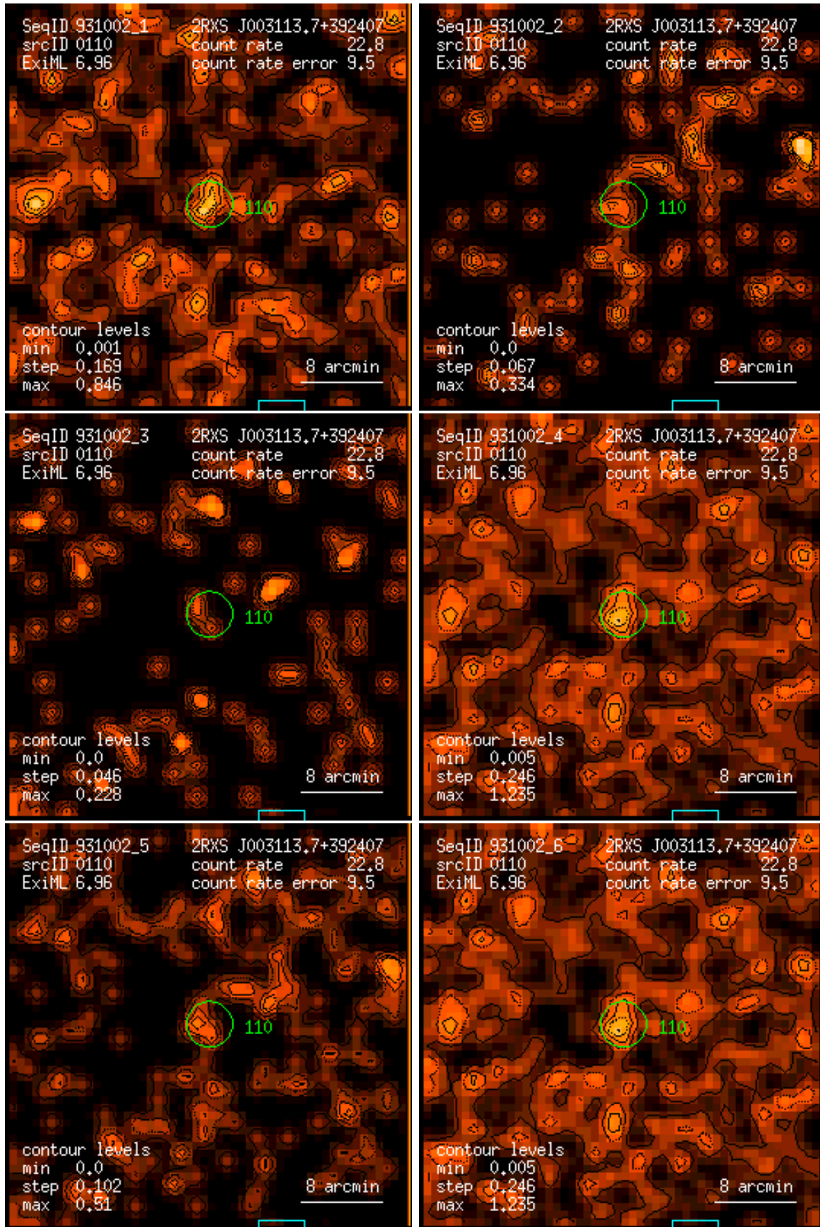
Figure 110: RASS 931002: detection 0110: band rate images, Gaussian filter: (1) PSPC channels 11 – 41, (2) 52 – 90, (3) 91 – 201, (4) 11 – 235, (5) 52 – 201, (6) 11 – 201. Broad band rates in counts/ks. Band rate contour levels in counts/ks/arcmin 2 .
