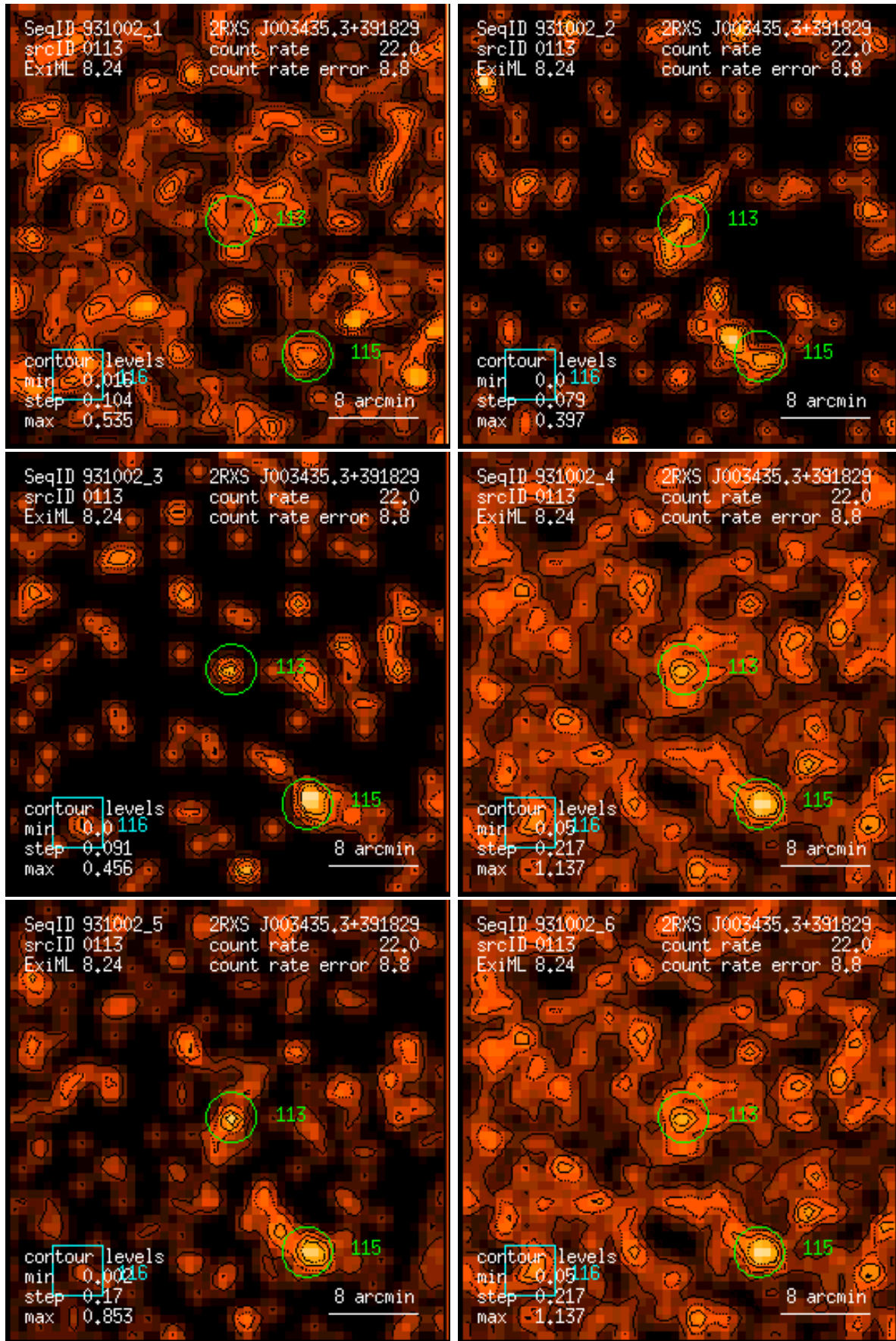
Figure 113: RASS 931002: detection 0113: band rate images, Gaussian filter: (1) PSPC channels 11 – 41, (2) 52 – 90, (3) 91 – 201, (4) 11 – 235, (5) 52 – 201, (6) 11 – 201. Broad band rates in counts/ks. Band rate contour levels in counts/ks/arcmin 2 .
