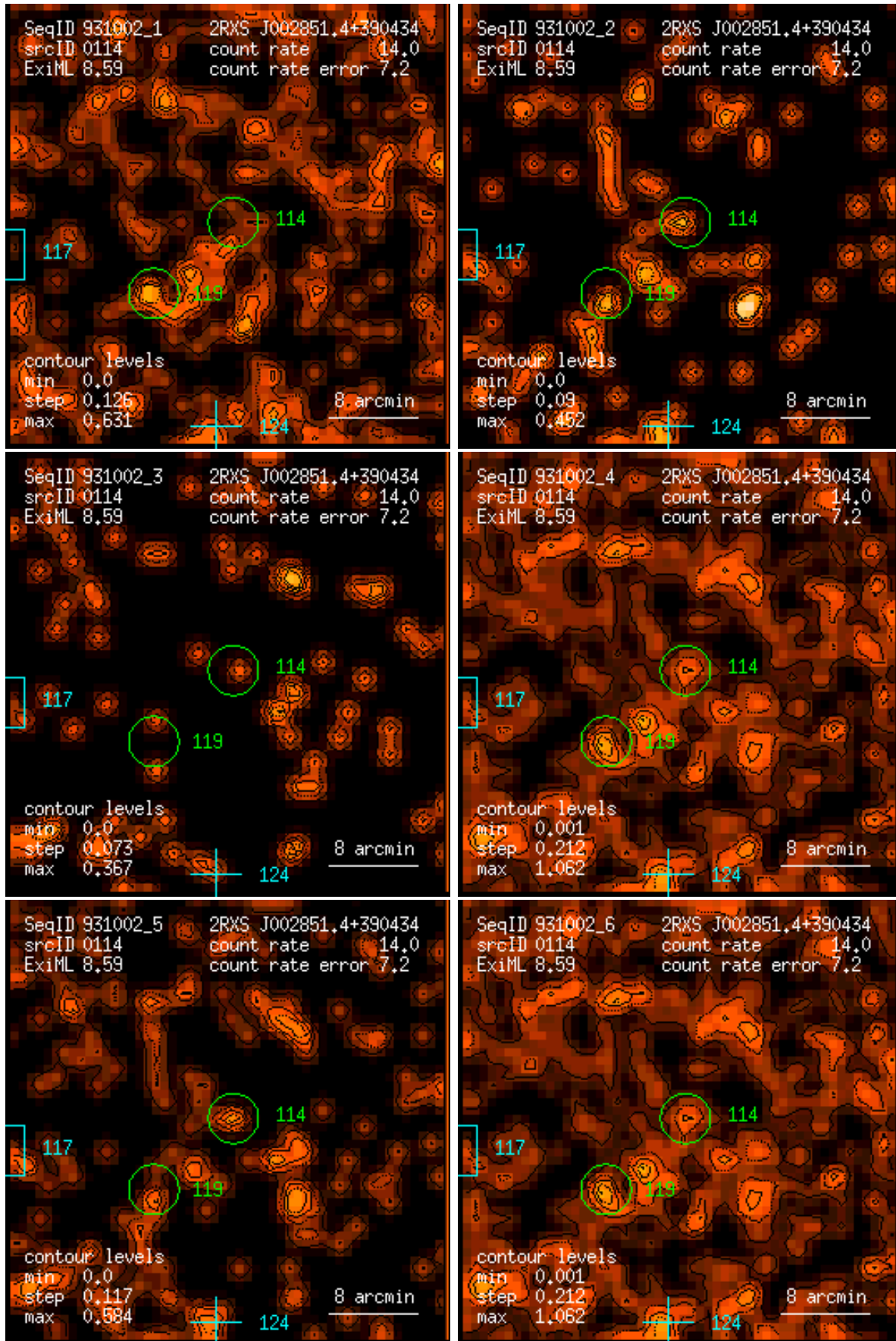
Figure 114: RASS 931002: detection 0114: band rate images, Gaussian filter: (1) PSPC channels 11 – 41, (2) 52 – 90, (3) 91 – 201, (4) 11 – 235, (5) 52 – 201, (6) 11 – 201. Broad band rates in counts/ks. Band rate contour levels in counts/ks/arcmin 2 .
