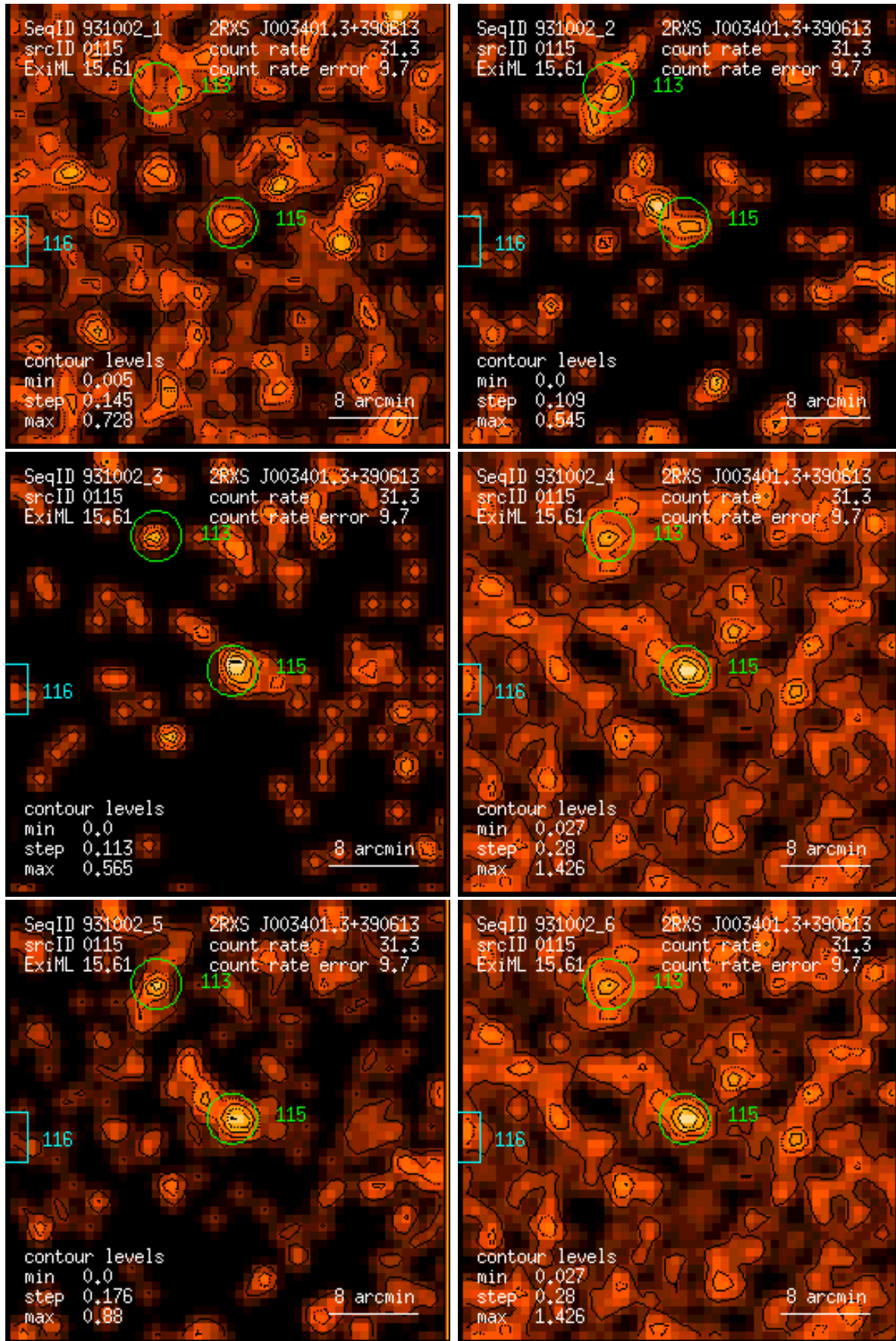
Figure 115: RASS 931002: detection 0115: band rate images, Gaussian filter: (1) PSPC channels 11 – 41, (2) 52 – 90, (3) 91 – 201, (4) 11 – 235, (5) 52 – 201, (6) 11 – 201. Broad band rates in counts/ks. Band rate contour levels in counts/ks/arcmin 2 .
