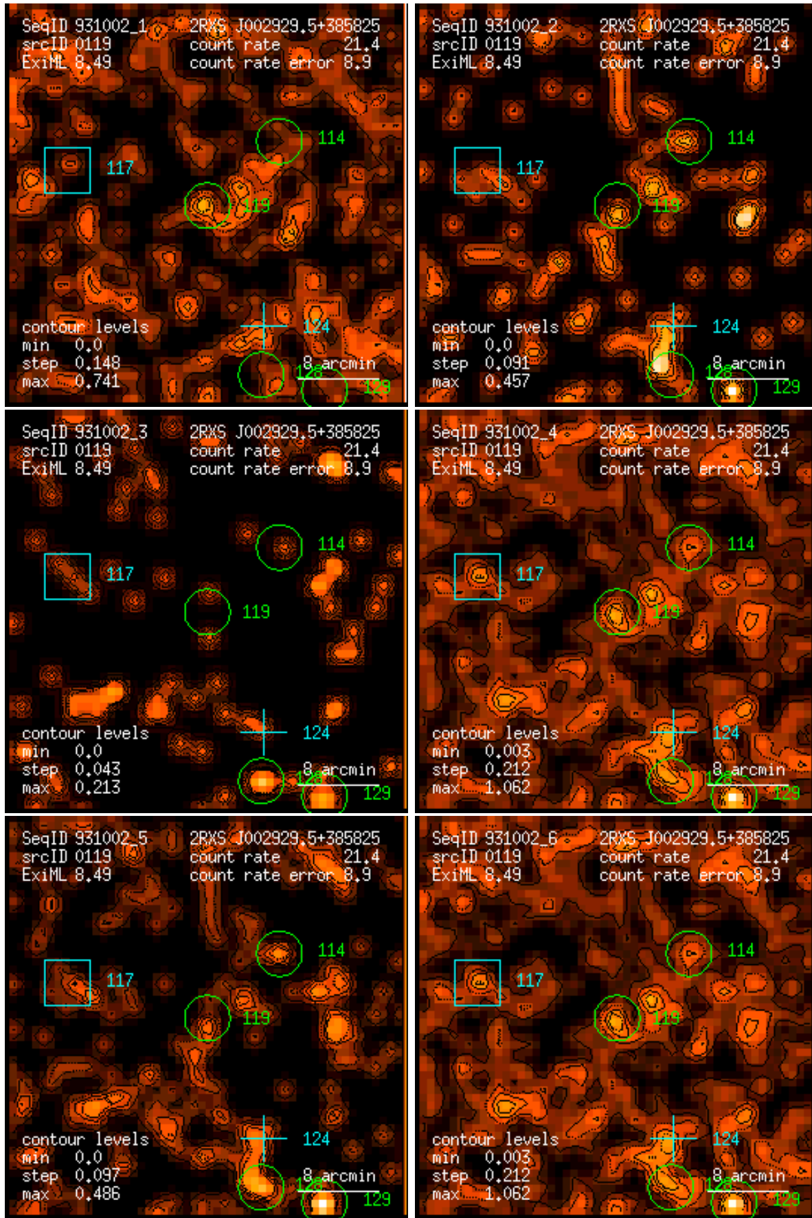
Figure 119: RASS 931002: detection 0119: band rate images, Gaussian filter: (1) PSPC channels 11 – 41, (2) 52 – 90, (3) 91 – 201, (4) 11 – 235, (5) 52 – 201, (6) 11 – 201. Broad band rates in counts/ks. Band rate contour levels in counts/ks/arcmin 2 .
