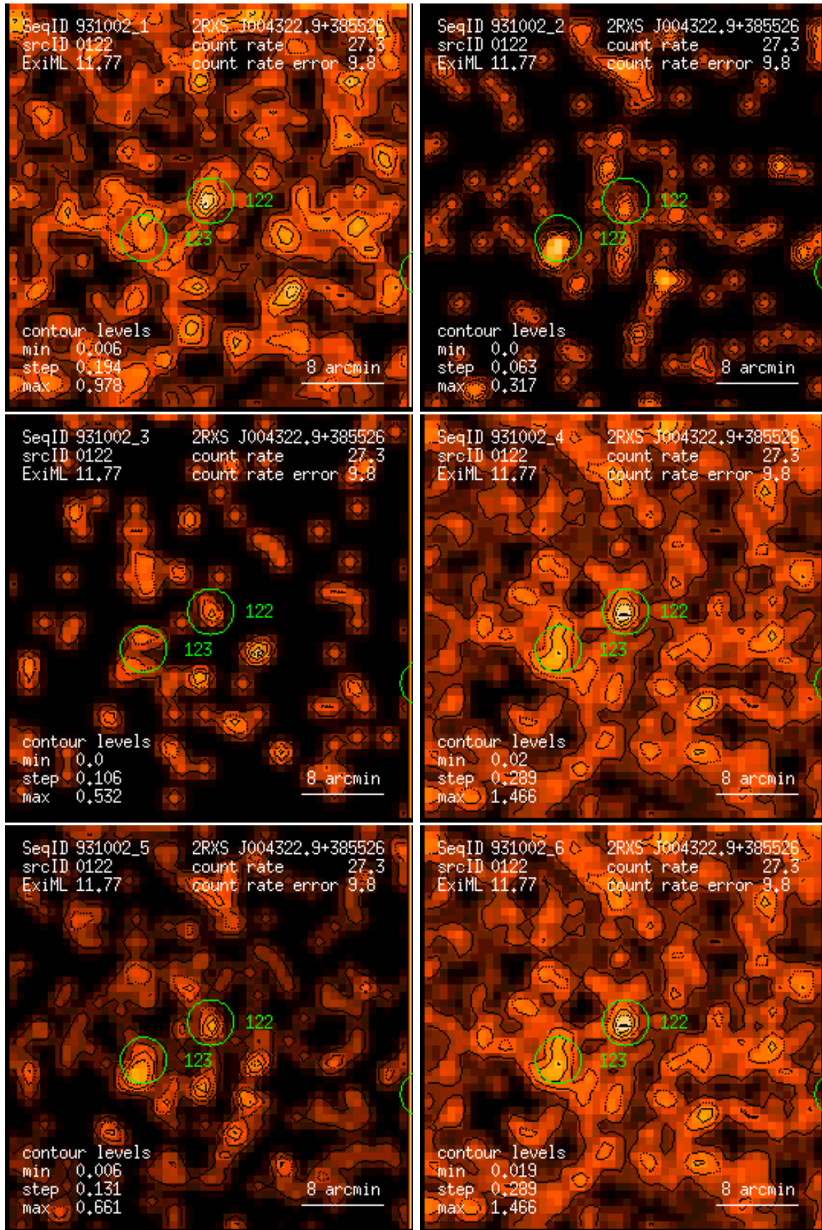
Figure 122: RASS 931002: detection 0122: band rate images, Gaussian filter: (1) PSPC channels 11 – 41, (2) 52 – 90, (3) 91 – 201, (4) 11 – 235, (5) 52 – 201, (6) 11 – 201. Broad band rates in counts/ks. Band rate contour levels in counts/ks/arcmin 2 .
