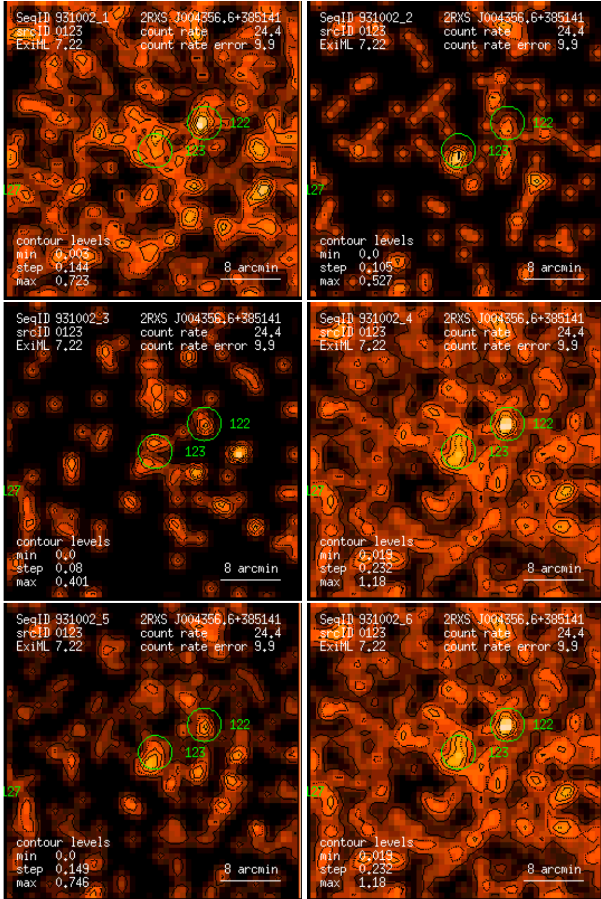
Figure 123: RASS 931002: detection 0123: band rate images, Gaussian filter: (1) PSPC channels 11 – 41, (2) 52 – 90, (3) 91 – 201, (4) 11 – 235, (5) 52 – 201, (6) 11 – 201. Broad band rates in counts/ks. Band rate contour levels in counts/ks/arcmin 2 .
