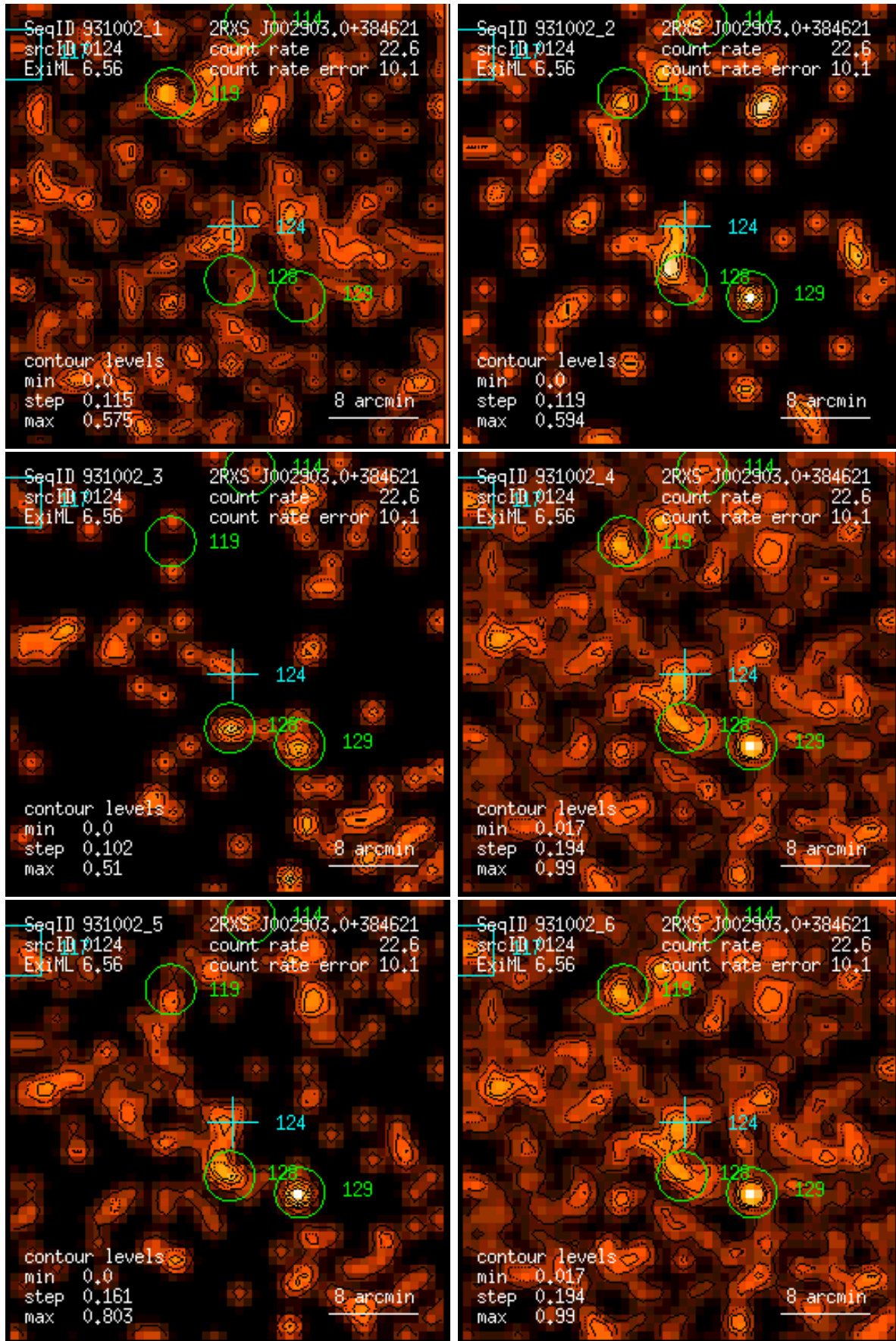
Figure 124: RASS 931002: detection 0124: band rate images, Gaussian filter: (1) PSPC channels 11 – 41, (2) 52 – 90, (3) 91 – 201, (4) 11 – 235, (5) 52 – 201, (6) 11 – 201. Broad band rates in counts/ks. Band rate contour levels in counts/ks/arcmin 2 .
