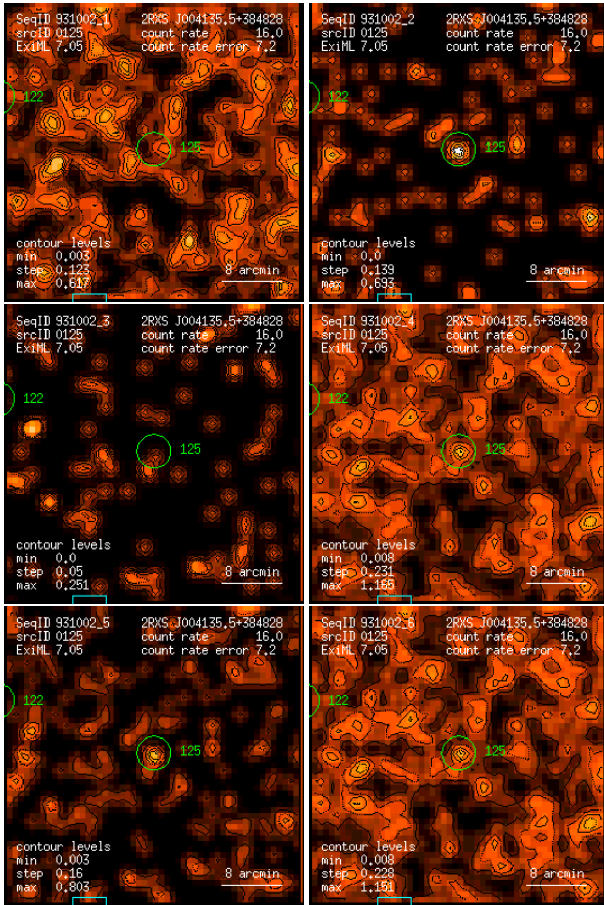
Figure 125: RASS 931002: detection 0125: band rate images, Gaussian filter: (1) PSPC channels 11 – 41, (2) 52 – 90, (3) 91 – 201, (4) 11 – 235, (5) 52 – 201, (6) 11 – 201. Broad band rates in counts/ks. Band rate contour levels in counts/ks/arcmin 2 .
