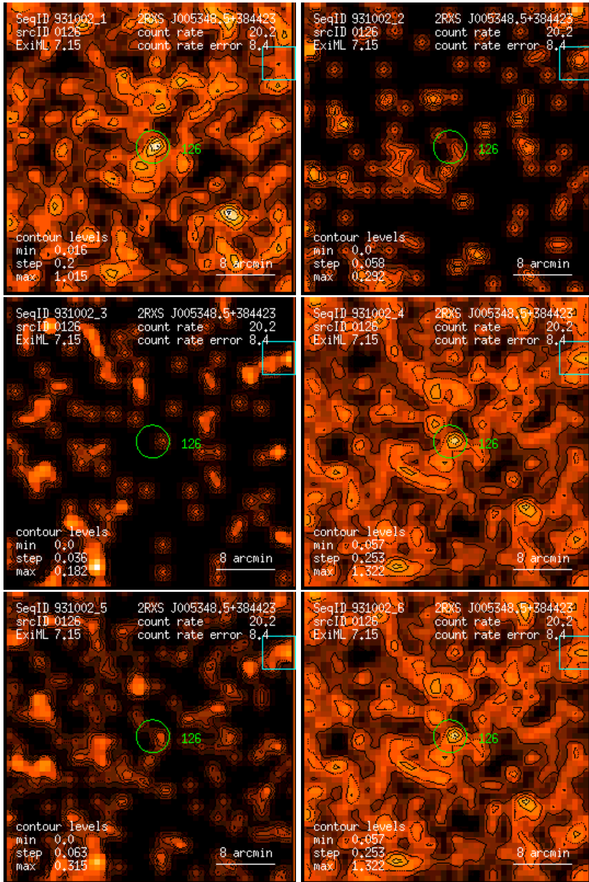
Figure 126: RASS 931002: detection 0126: band rate images, Gaussian filter: (1) PSPC channels 11 – 41, (2) 52 – 90, (3) 91 – 201, (4) 11 – 235, (5) 52 – 201, (6) 11 – 201. Broad band rates in counts/ks. Band rate contour levels in counts/ks/arcmin 2 .
