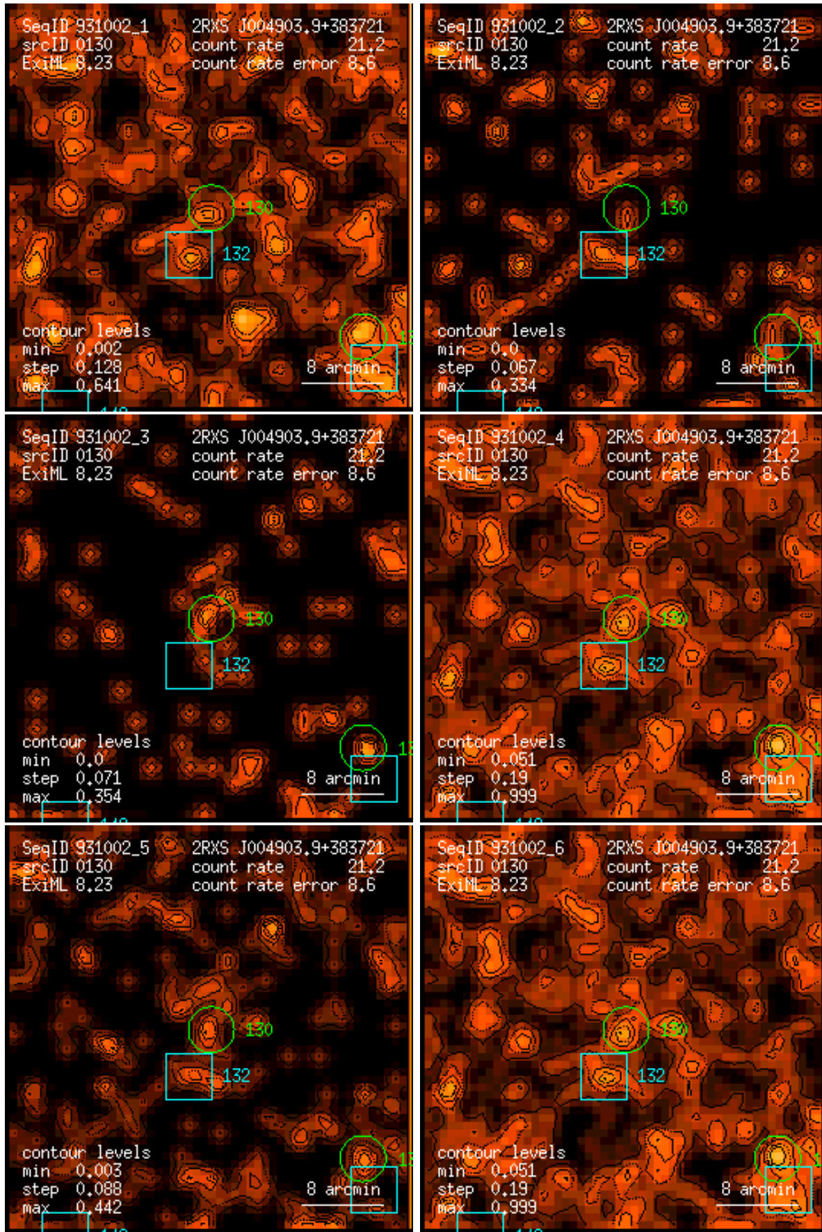
Figure 130: RASS 931002: detection 0130: band rate images, Gaussian filter: (1) PSPC channels 11 – 41, (2) 52 – 90, (3) 91 – 201, (4) 11 – 235, (5) 52 – 201, (6) 11 – 201. Broad band rates in counts/ks. Band rate contour levels in counts/ks/arcmin 2 .
