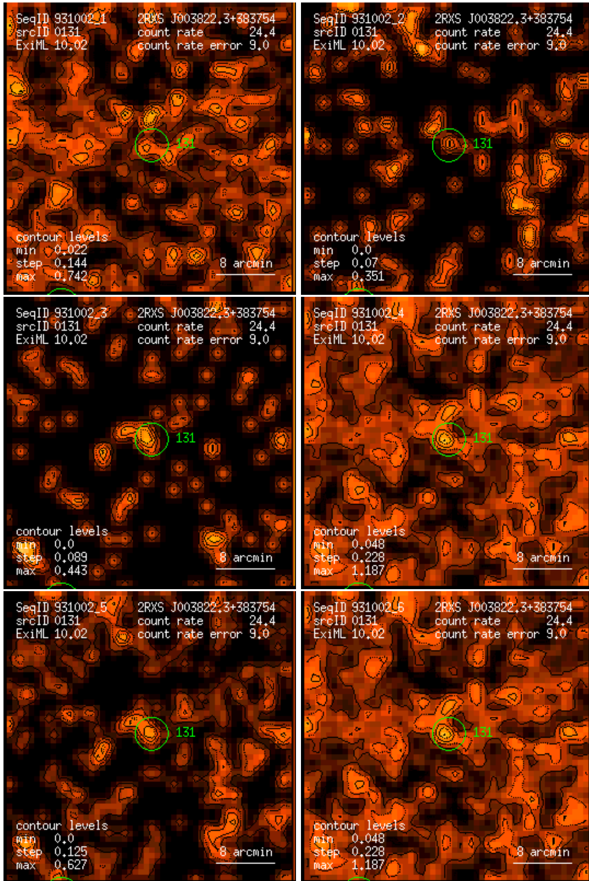
Figure 131: RASS 931002: detection 0131: band rate images, Gaussian filter: (1) PSPC channels 11 – 41, (2) 52 – 90, (3) 91 – 201, (4) 11 – 235, (5) 52 – 201, (6) 11 – 201. Broad band rates in counts/ks. Band rate contour levels in counts/ks/arcmin 2 .
