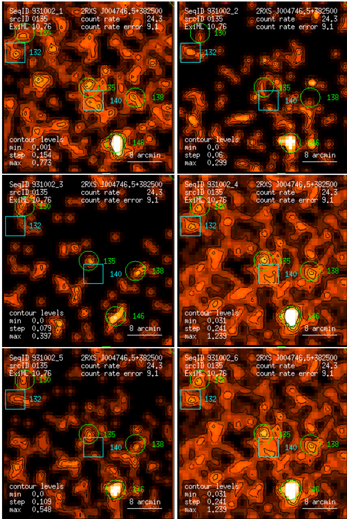
Figure 135: RASS 931002: detection 0135: band rate images, Gaussian filter: (1) PSPC channels 11 – 41, (2) 52 – 90, (3) 91 – 201, (4) 11 – 235, (5) 52 – 201, (6) 11 – 201. Broad band rates in counts/ks. Band rate contour levels in counts/ks/arcmin 2 .
