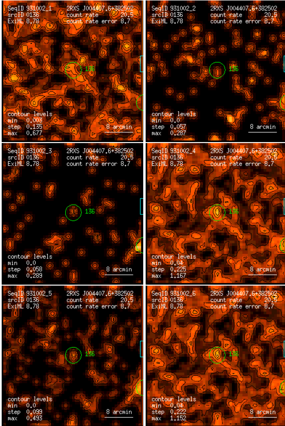
Figure 136: RASS 931002: detection 0136: band rate images, Gaussian filter: (1) PSPC channels 11 – 41, (2) 52 – 90, (3) 91 – 201, (4) 11 – 235, (5) 52 – 201, (6) 11 – 201. Broad band rates in counts/ks. Band rate contour levels in counts/ks/arcmin 2 .
