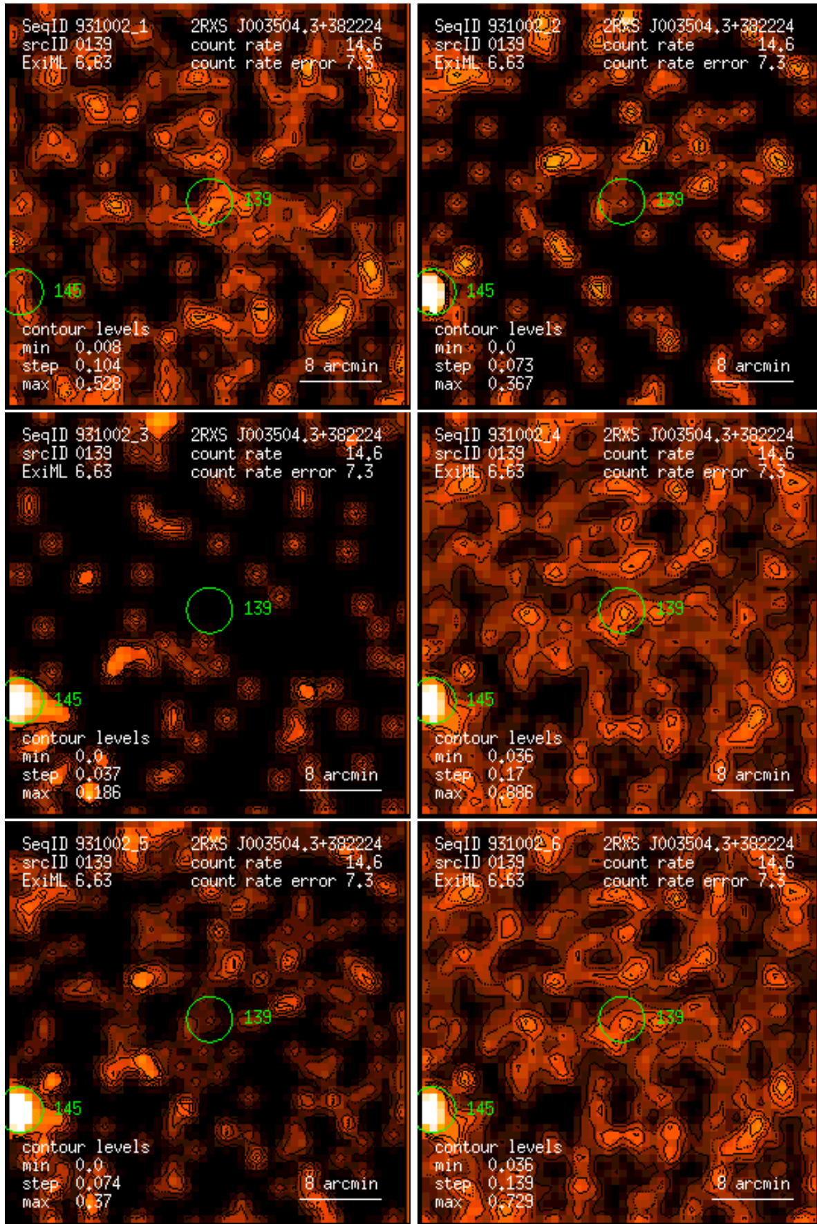
Figure 139: RASS 931002: detection 0139: band rate images, Gaussian filter: (1) PSPC channels 11 – 41, (2) 52 – 90, (3) 91 – 201, (4) 11 – 235, (5) 52 – 201, (6) 11 – 201. Broad band rates in counts/ks. Band rate contour levels in counts/ks/arcmin 2 .
