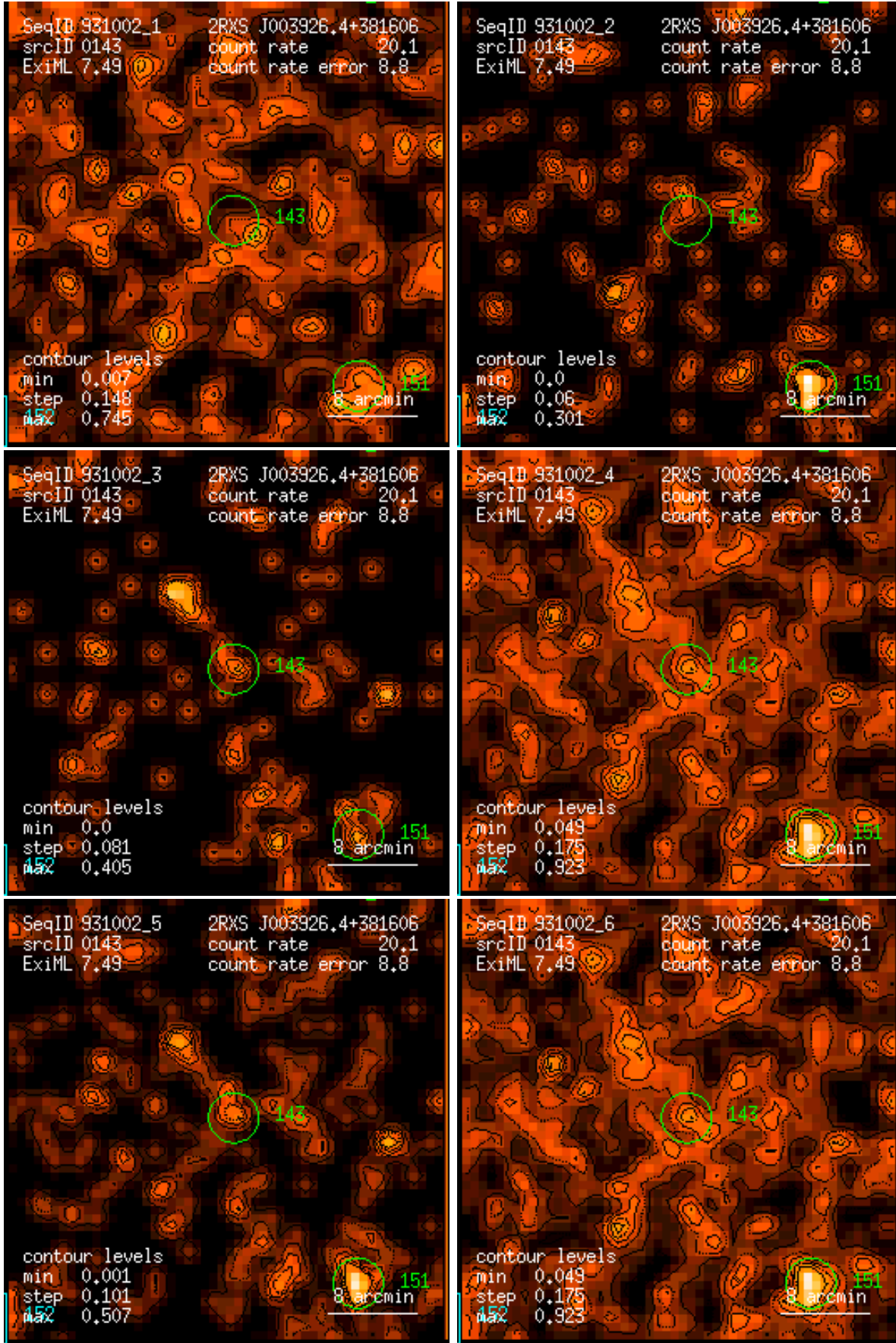
Figure 143: RASS 931002: detection 0143: band rate images, Gaussian filter: (1) PSPC channels 11 – 41, (2) 52 – 90, (3) 91 – 201, (4) 11 – 235, (5) 52 – 201, (6) 11 – 201. Broad band rates in counts/ks. Band rate contour levels in counts/ks/arcmin 2 .
