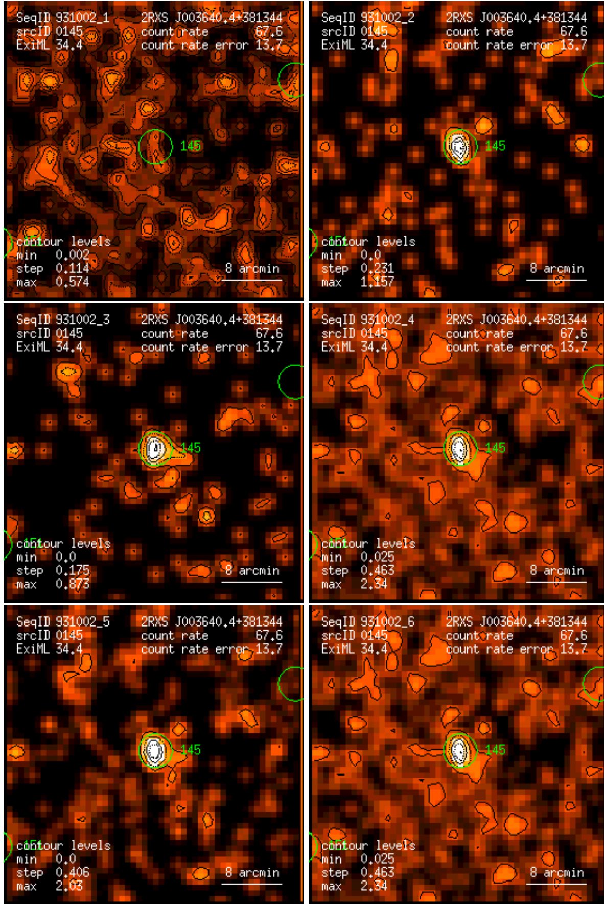
Figure 145: RASS 931002: detection 0145: band rate images, Gaussian filter: (1) PSPC channels 11 – 41, (2) 52 – 90, (3) 91 – 201, (4) 11 – 235, (5) 52 – 201, (6) 11 – 201. Broad band rates in counts/ks. Band rate contour levels in counts/ks/arcmin 2 .
