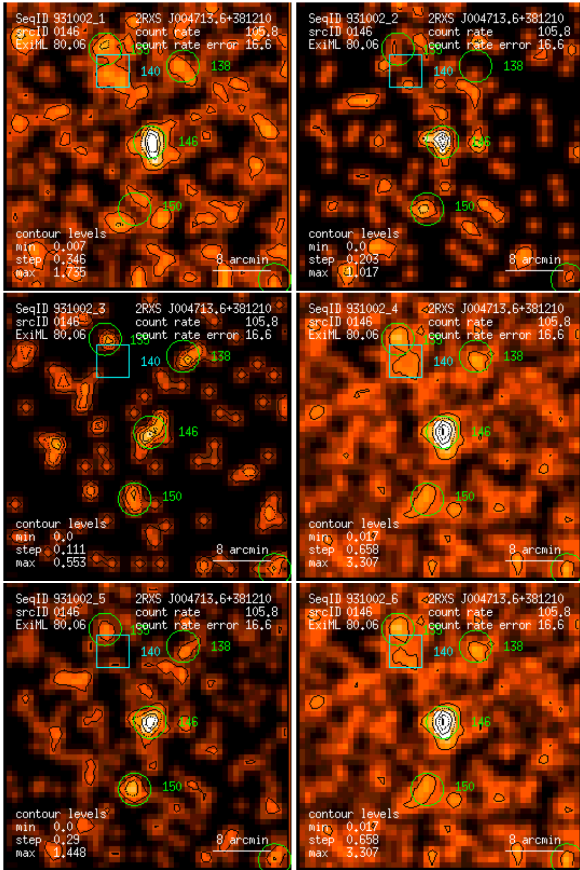
Figure 146: RASS 931002: detection 0146: band rate images, Gaussian filter: (1) PSPC channels 11 – 41, (2) 52 – 90, (3) 91 – 201, (4) 11 – 235, (5) 52 – 201, (6) 11 – 201. Broad band rates in counts/ks. Band rate contour levels in counts/ks/arcmin 2 .
