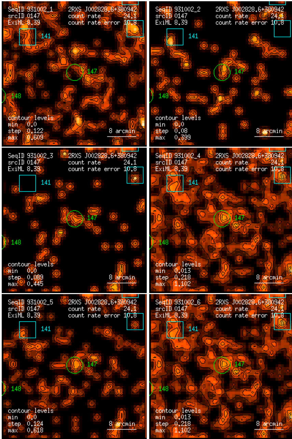
Figure 147: RASS 931002: detection 0147: band rate images, Gaussian filter: (1) PSPC channels 11 – 41, (2) 52 – 90, (3) 91 – 201, (4) 11 – 235, (5) 52 – 201, (6) 11 – 201. Broad band rates in counts/ks. Band rate contour levels in counts/ks/arcmin 2 .
