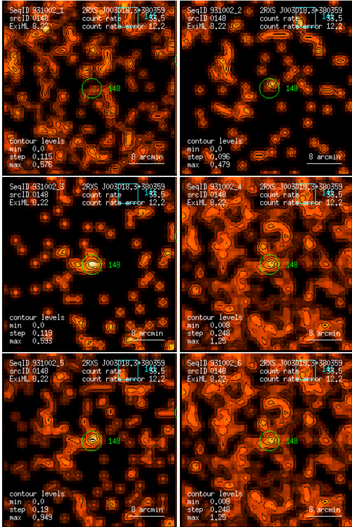
Figure 148: RASS 931002: detection 0148: band rate images, Gaussian filter: (1) PSPC channels 11 – 41, (2) 52 – 90, (3) 91 – 201, (4) 11 – 235, (5) 52 – 201, (6) 11 – 201. Broad band rates in counts/ks. Band rate contour levels in counts/ks/arcmin 2 .
