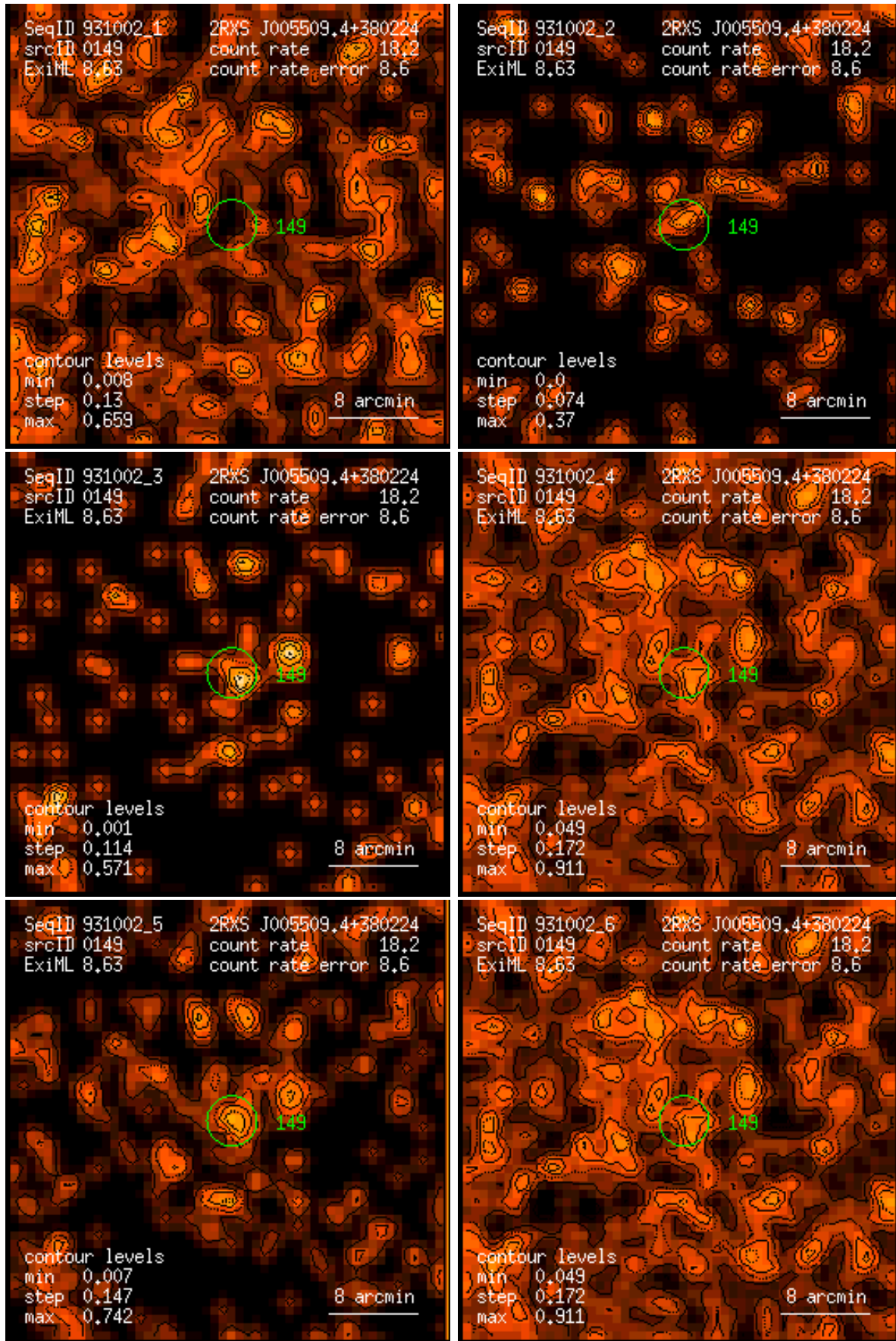
Figure 149: RASS 931002: detection 0149: band rate images, Gaussian filter: (1) PSPC channels 11 – 41, (2) 52 – 90, (3) 91 – 201, (4) 11 – 235, (5) 52 – 201, (6) 11 – 201. Broad band rates in counts/ks. Band rate contour levels in counts/ks/arcmin 2 .
